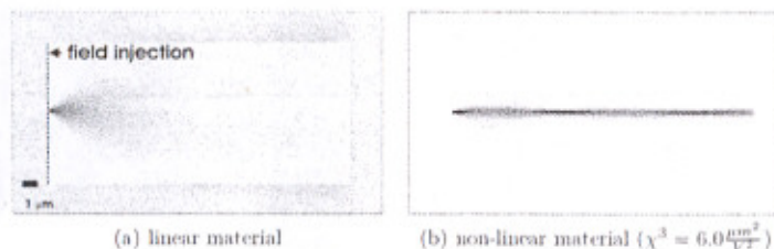
Fig. 1. Injecting a Gaussian bundle in a non-linear Kerr material results in a soliton.
