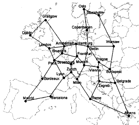
Fig. 2. Pan-European fiber-optic network topology
