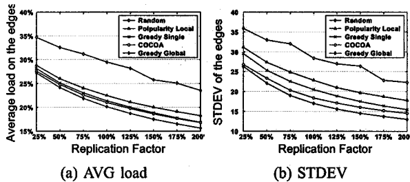
Fig. 5. Average load and STDEV without TE
