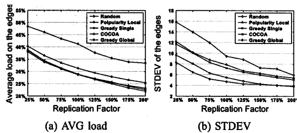
Fig. 7. Average load and STDEV with TE
