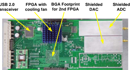
Figure 4 : Single Digital Module
