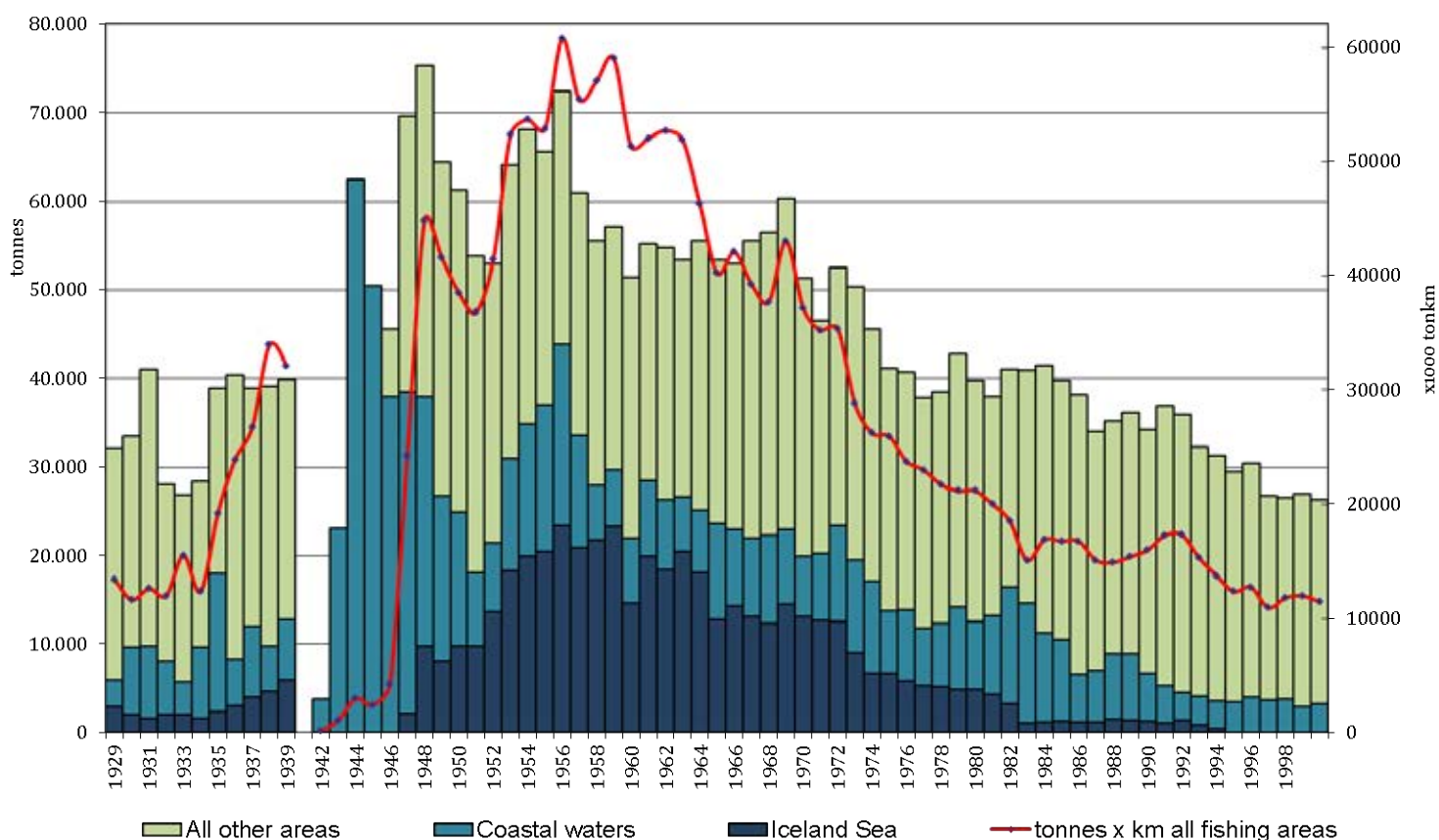
Figure 4.9.: The annual tonne-kilometres of the Belgian sea fisheries, red line (values in right-hand axis), calculated as the sum of the annual landings per fishing area a (tonnes) multiplied by the km distance to the centre of the fishing area a . The columns represent the overall annual landings per year (tonnes, left-hand axis) for the distant 'Iceland Sea' (dark blue), the nearby 'Coastal waters' (median blue) and the remaining reported areas as 'all other areas' (light green).
