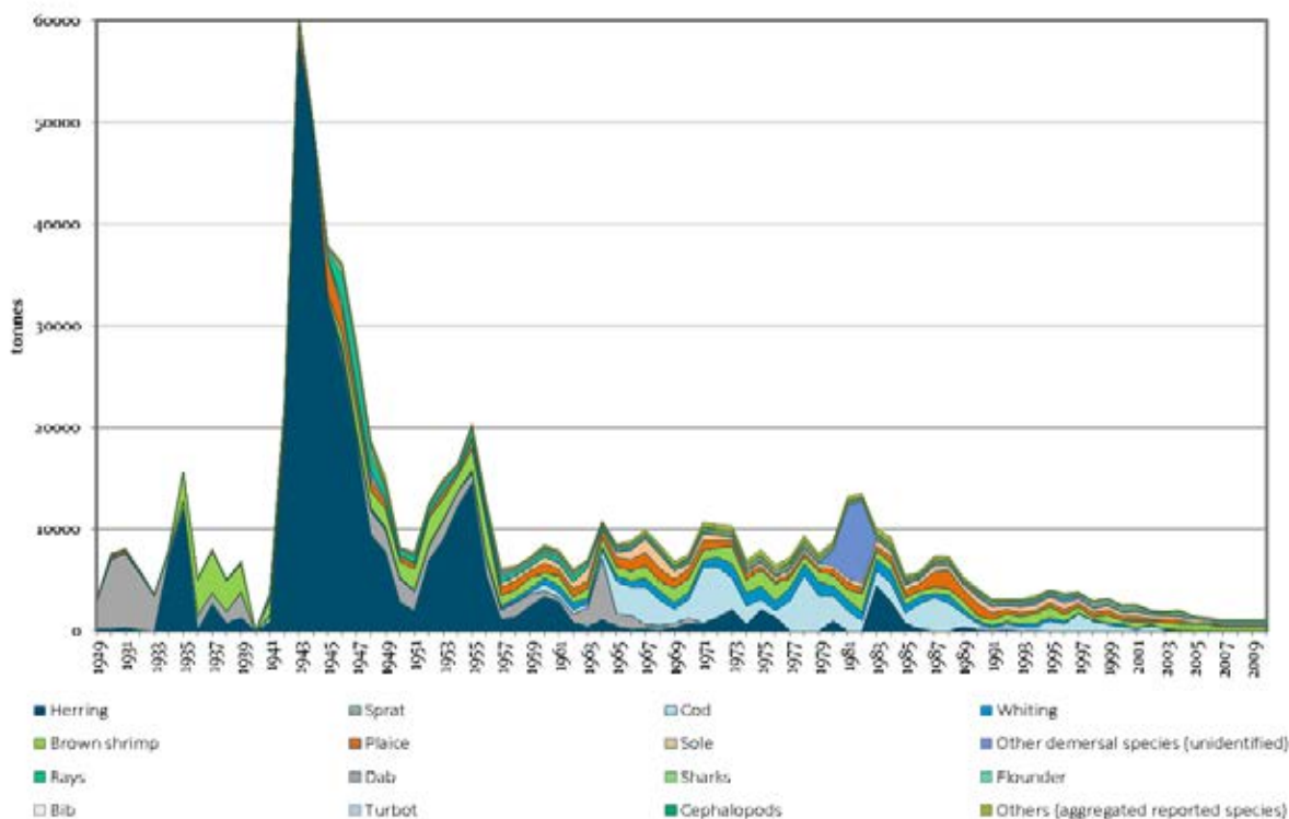
Figure 4.12.: Annual landings from the Coastal waters, by species. Based on annual landings in Belgium and in foreign ports
