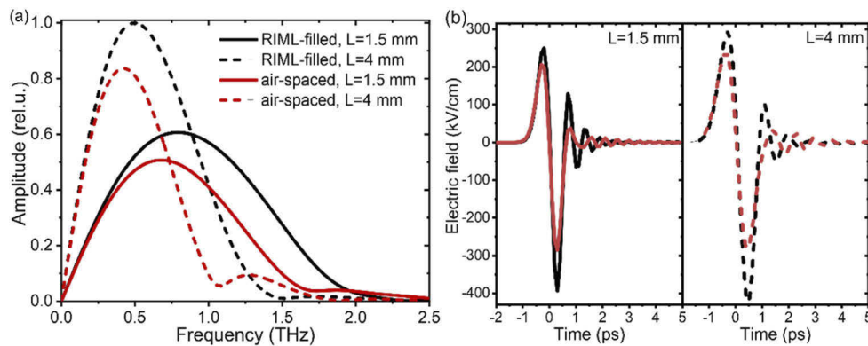
Fig. 4. Calculated amplitude spectra (a) and electric-field waveforms (b) of the air-spaced (red lines) and RIML-filled (black lines) setups, at 1.5 mm (solid lines) and 4 mm (dashed lines) NLES thicknesses.
