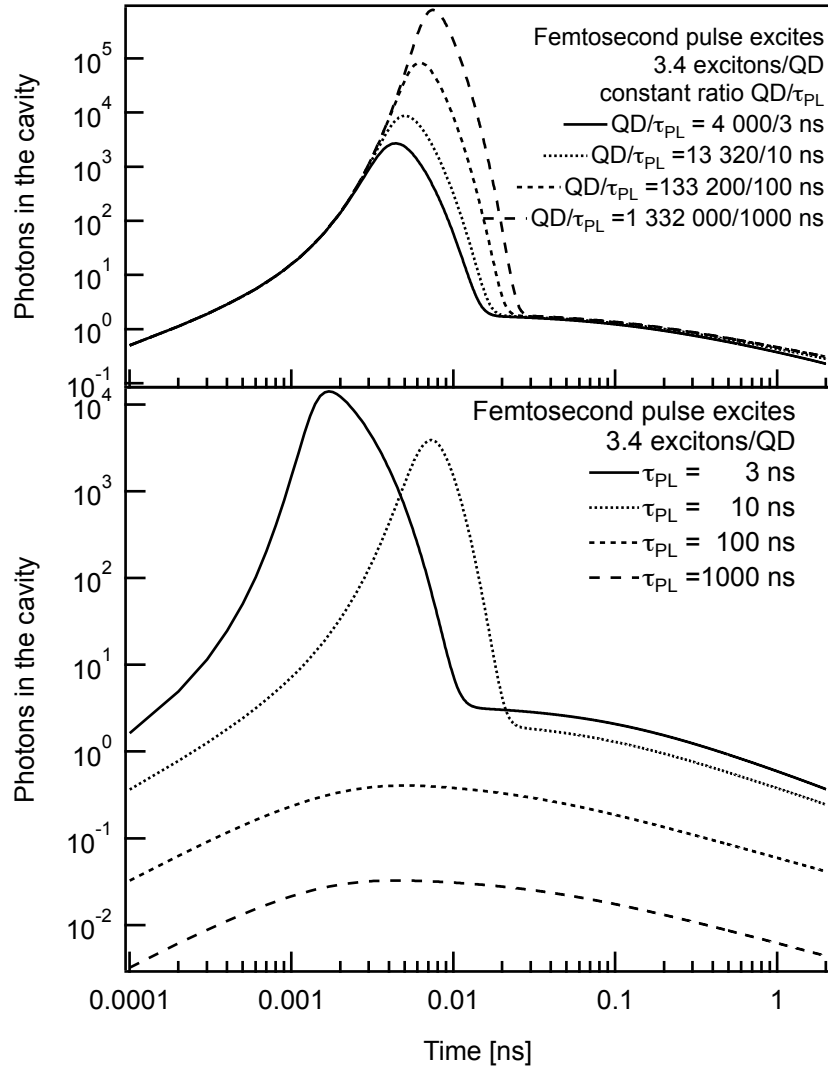
Figure 7.8: (top) Number of photons \phi in a certain cavity mode as a function of time for different values of the \tau_{PL} , while keeping the modal gain N_{QD}/\tau_{PL} constant, shows that lower QD gain results in a higher peak energy and larger pulse width. (bottom) Idem, for different values of the modal gain or \tau_{PL} shows that enough modal gain is necessary to overcome non-radiative losses.
