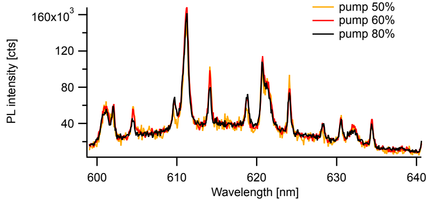
Figure 8.22: Spectrum of a 7.5 \mu\text{m} microdisk, containing 30 nm thick layer of SILAR CdSe/CdS/ZnS QDs, using a 600 lines/mm grating for three different pump powers of the excitation laser, normalized to the background emission shows the linear increase of the output spectrum.
