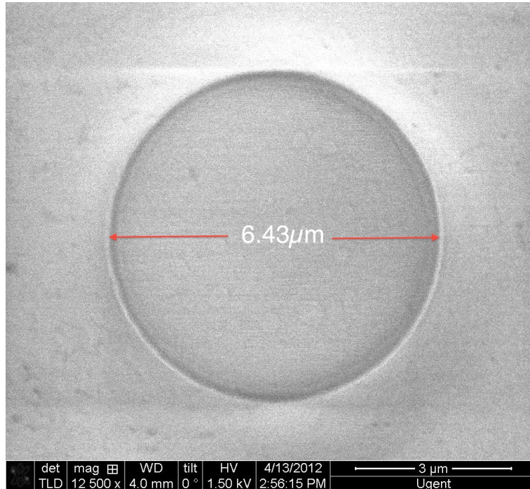
Figure 8.11: The diameter of the indicated microdisk measured using SEM is larger than the designed diameter of 6.0 \mu\text{m} .
