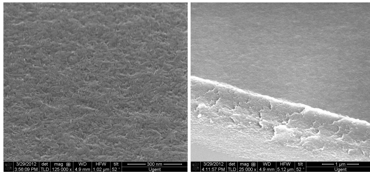
Figure 8.10: SEM of a spincoated layer of QRods (4.5 nm by 22.3 nm) of 28 nm thickness. The image on the left shows the morphology and local structuring of the rods in the spincoated layer. The right image shows the cut in the layer made using a doctor blade to measure the thickness using AFM. It shows the smoothness of the layer.
