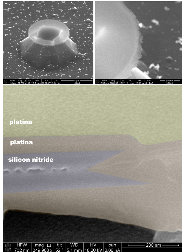
Figure 8.2: (a) Microdisk etched after QD and low-index \text{Si}_3\text{N}_4 deposition shows a diffuse edge, eaten away by KOH. (b) The brittle edge is clearer at higher magnification (c) A cross section of the microdisk shows that the QDs and part of \text{Si}_3\text{N}_4 has been etched away by KOH. Deeper in the layer voids are visible where QDs were etched away.
