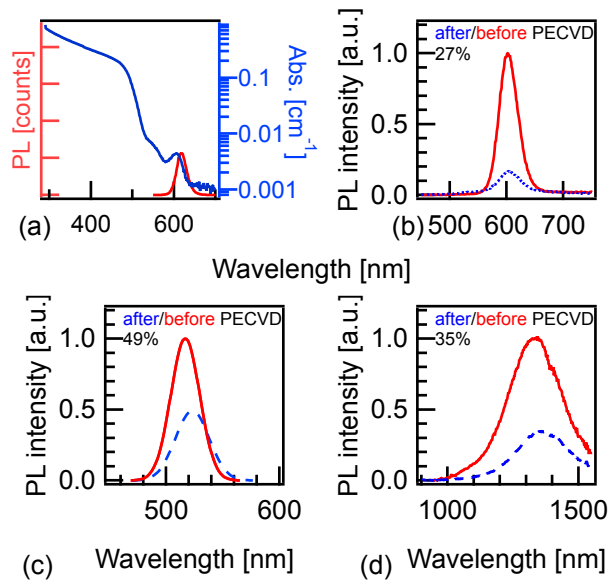
Figure 8.14: (a) PL (red) and absorption (blue) spectrum of 12 nm giant CdSe/14CdS QDs used in the microdisk experiment. (b) PL spectrum of spincoated CdSe/16CdS QDs before (red) and after (blue) deposition of low-index \text{Si}_3\text{N}_4 (see Section 8.2.1) shows that 27% of the emission remains after \text{Si}_3\text{N}_4 deposition. (c) A similar experiment for CdSe/2ZnS QDs illustrates that 50% of the PL remains after deposition. (d) Also for near-infrared emitting PbS/CdS QDs 35% of the PL is recovered after \text{Si}_3\text{N}_4 deposition.
