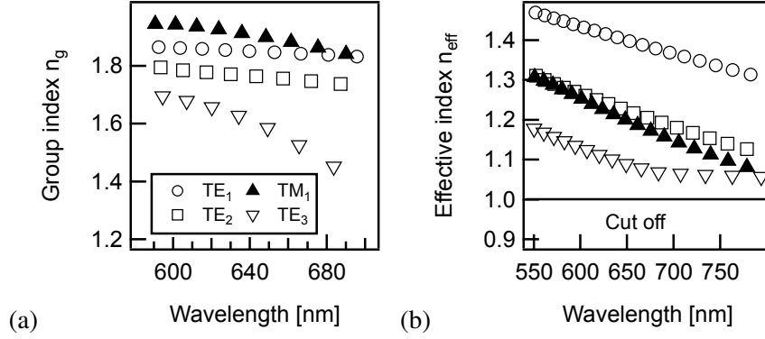
Figure 7.6: (a) Group index n_g and (b) effective index n_{\text{eff}} for a 5.5 \mu\text{m} microdisk for the first four modes
