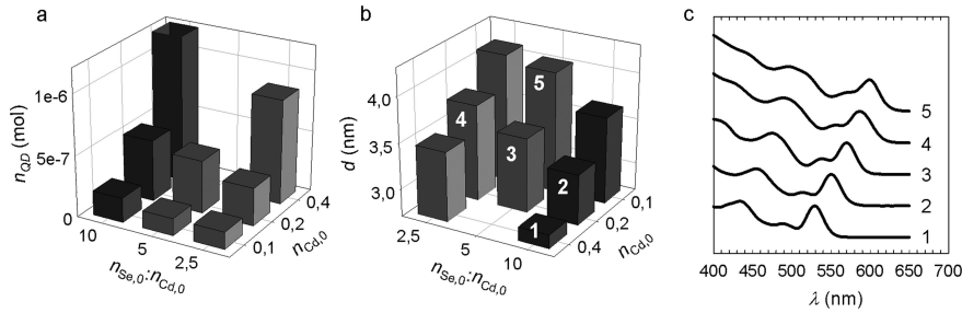
Figure 2.12: (a) Concentration of QDs formed as a function of n_{Cd,0} and the n_{Se,0}:n_{Cd,0} ratio; 280 °C /260 °C injection/growth temperature. (b) Postfocused diameter obtained as a function of n_{Cd,0} and the n_{Se,0}:n_{Cd,0} ratio. Note that the direction of each axis is swapped with respect to (a). (c) Absorption spectrum corresponding to the samples as indicated in (b).
