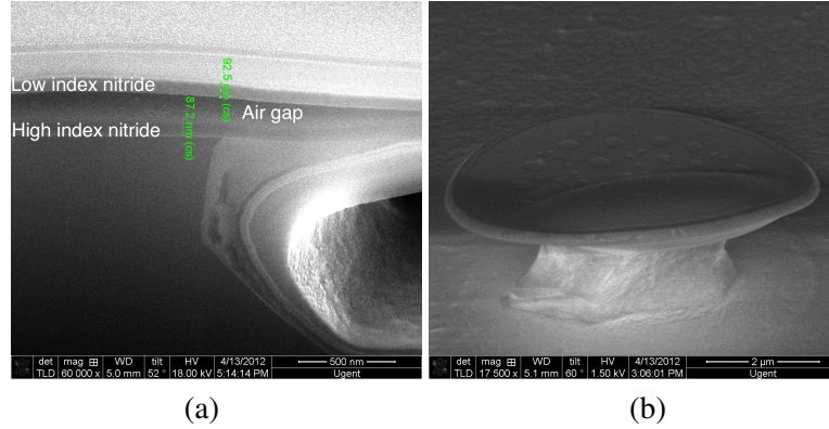
Figure 8.12: (a) Cross section using SEM shows how the bottom and top \text{Si}_3\text{N}_4 layer have detached under SEM electron bombardment. (b) The microdisk inflates or blows up under SEM.
