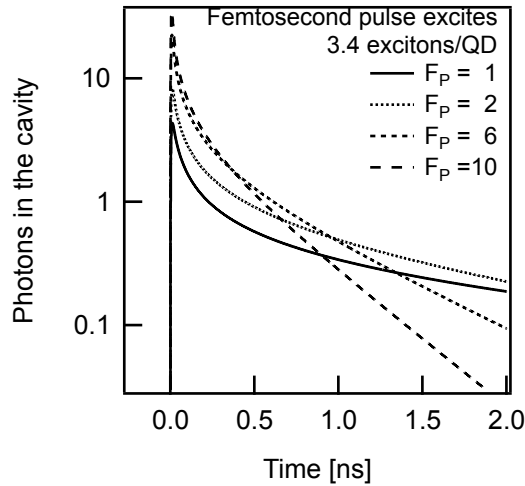
Figure 8.32: Simulated decay curve of a microdisk excited with a pulse of 3.4 excitons/QD for different Purcell factors shows the Purcell effect at high pump fluences.
