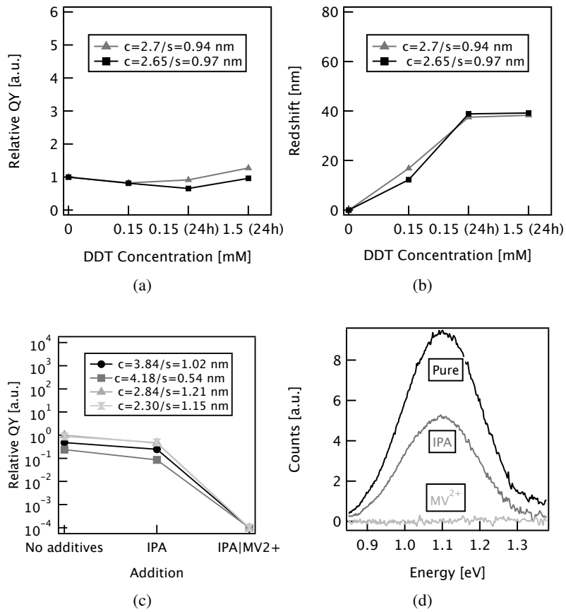
Figure 5.5: (a) Relative QY and (b) PL redshift before and after adding thiols (c) Relative QY (log-scale) and (d) PL spectra before and after adding IPA and MV 2+ /IPA. The graphs show the clear difference between the addition of a hole acceptor and an electron acceptor to PbSe/CdSe QDs.
