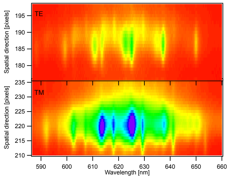
Figure 8.20: Mode map of a 6.0 \mu\text{m} microdisk for the TE polarization (top) and TM polarization (bottom)
