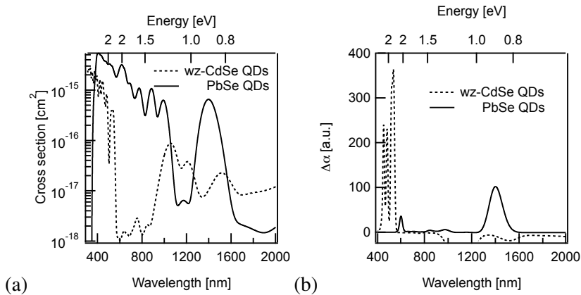
Figure 6.11: (a) The absorption cross section for wurtzite (wz) CdSe QDs and PbSe QDs with a diameter of 4.5 nm, as calculated by tight-binding and corrected for the local field factor in C_2Cl_4 (0.339 and 0.059 for CdSe and PbSe resp.) (b) Differential absorption, normalized to the intraband absorption directly below the band gap (600 nm for wz-CdSe, 1700 nm for PbSe) shows the higher contrast of the AB and PA expected for CdSe as compared to PbSe.
