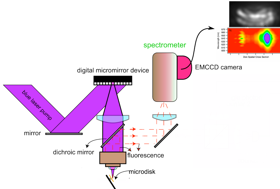
Figure 8.17: Selective Excitation Setup for Spatial and Spectral Imaging at the ULB shows the laser beam incident on the DMD. A pixel on the DMD is imaged onto the sample plane by a 100x objective. The PL is collected using the same lens and sent to a dichroic mirror. An image of the sample is formed on the entrance slit of the spectrometer, which can be used to collect a spatial image of the microdisk (top graph) or hybrid spatial/spectral image (bottom graph)
