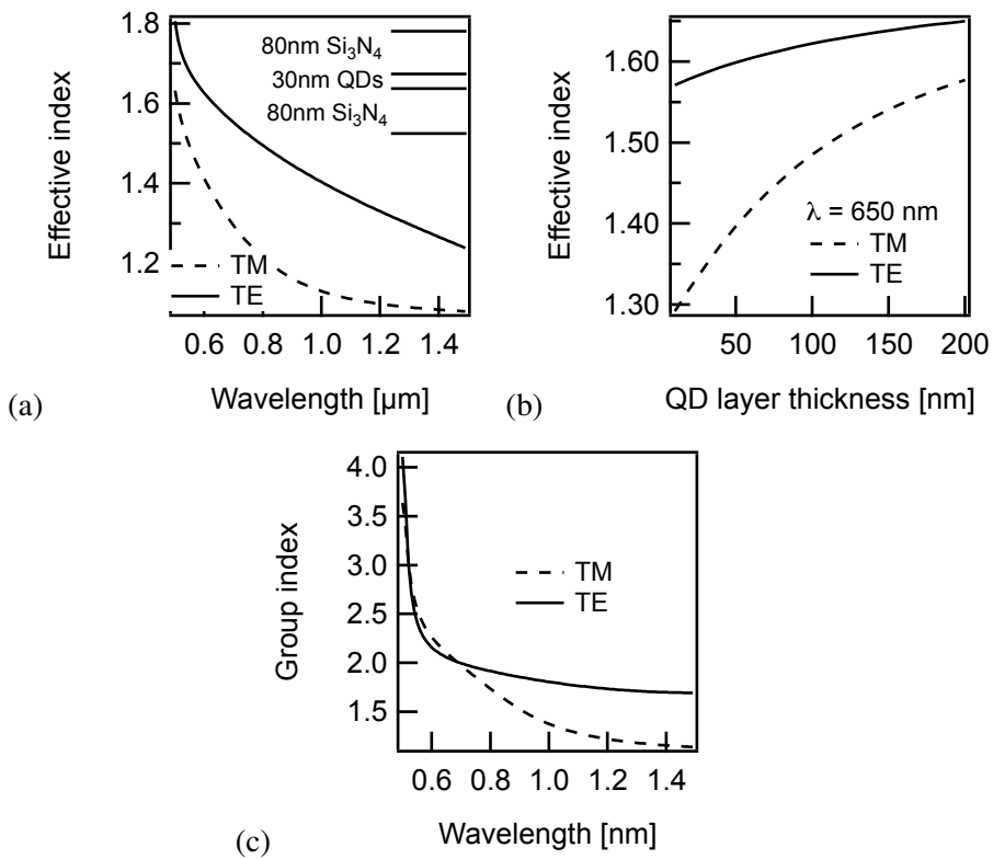
Figure 7.1: (a) The dispersion of the effective index for a slab waveguide with the layer stack as drawn above. (b) The effective index for different thickness of the QD layer. (c) The group index n_g as a function of wavelength.
