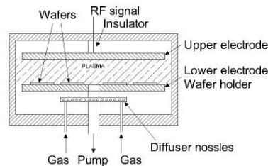
Figure 8.5: The layout of the RIE machine shows the parallel plates, with the drifting plasma in between.
