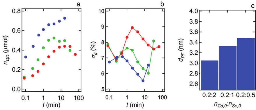
Figure 2.11: (a) Time evolution of the amount of QDs for reactions with n_{Cd,0}:n_{Se,0} of (blue) 0.2:2, (green) 0.2:1, and (red) 0.2:0.5 (numbers in mmol), 245 °C /230 °C injection/growth temperature. (b) Time evolution of the size dispersion for the same reactions as in (a). (c) Postfocused diameter of the different reactions.
