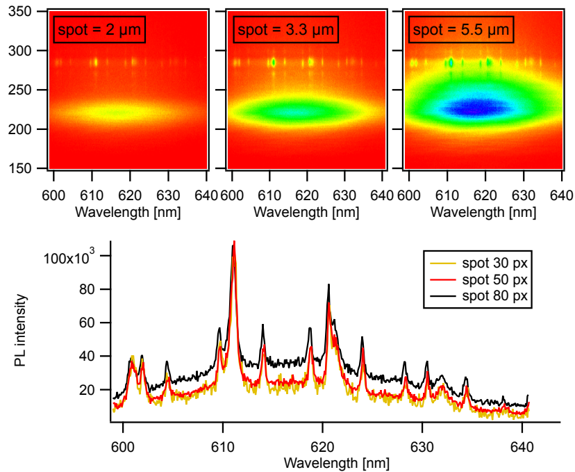
Figure 8.21: (a) Mode maps of a 6.5 \mu\text{m} microdisk, containing 30 \text{ nm} thick layer of SILAR CdSe/CdS/ZnS QDs, using a 600 \text{ lines/mm} grating for three different excitation spot sizes ( 2 , 3.3 and 5.5 \mu\text{m} ). All maps are shown on the same scale, so the emission intensities can be compared. (b) Spectrum for the different spot sizes by normalizing the peak intensities shows the faster growth of the background emission.
