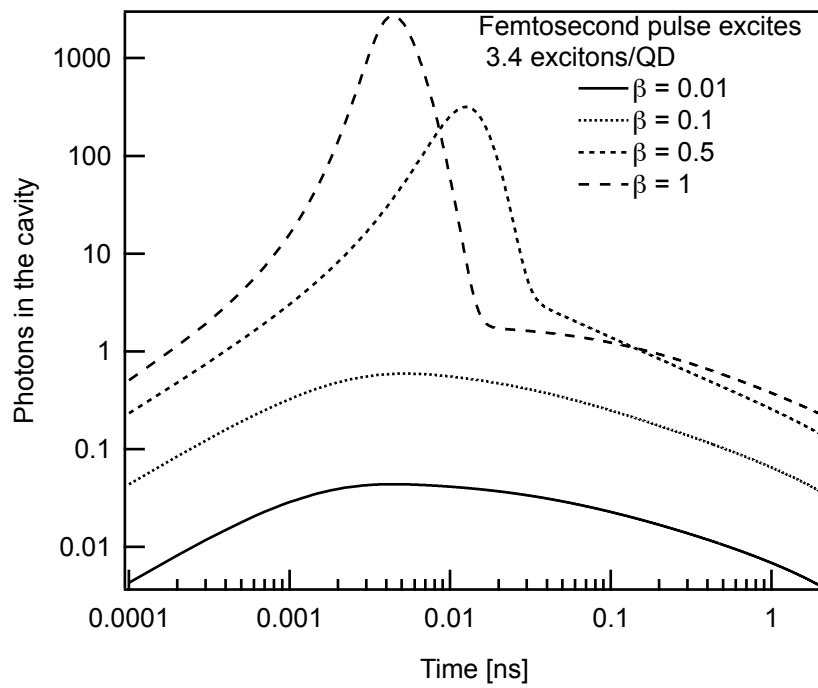
Figure 7.11: Number of photons \phi in a certain cavity mode as a function of time for different values of the spontaneous emission coupling factor \beta shows that the laser pulse disappears for lower \beta , mainly due to the lower modal gain.
