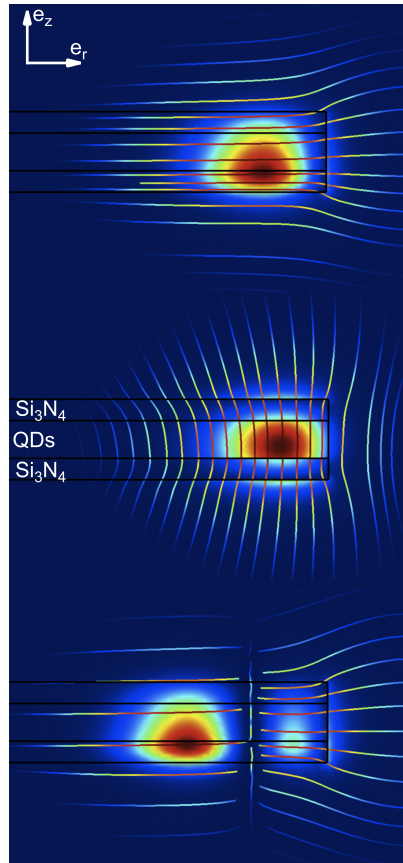
Figure 8.19: Field lines \mathbf{E}_t = E_r \mathbf{e}_r + E_z \mathbf{e}_z for the TE 1 (top), TM 1 (middle) and TE 2 (bottom) modes, plotted against the background of the mode intensity |\mathbf{E}|^2 , show that both modes are hybrid, especially at the corners of the structure.
