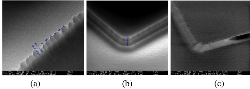
Figure 8.6: RIE of 80 nm of \text{Si}_3\text{N}_4 on top of a silicon substrate. From left to right, the gas mixture is changed: \text{SF}_6:\text{O}_2 (a) 50:30 sccm (b) 30:30 sccm (c) 5:30 sccm. The etching mechanism goes from chemical, over synergetic to full physical etching.
