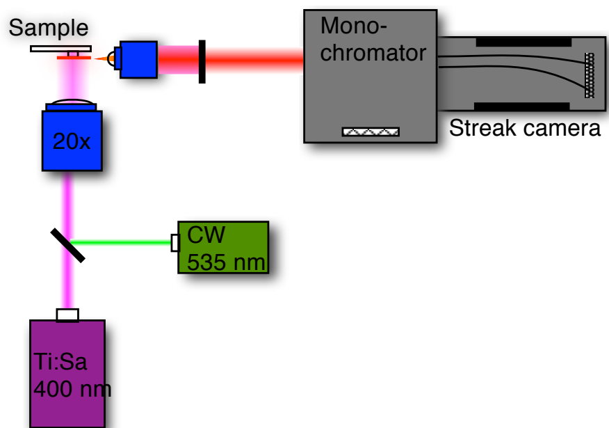
Figure 8.23: Microdisk pump setup used in Trento, Italy.
