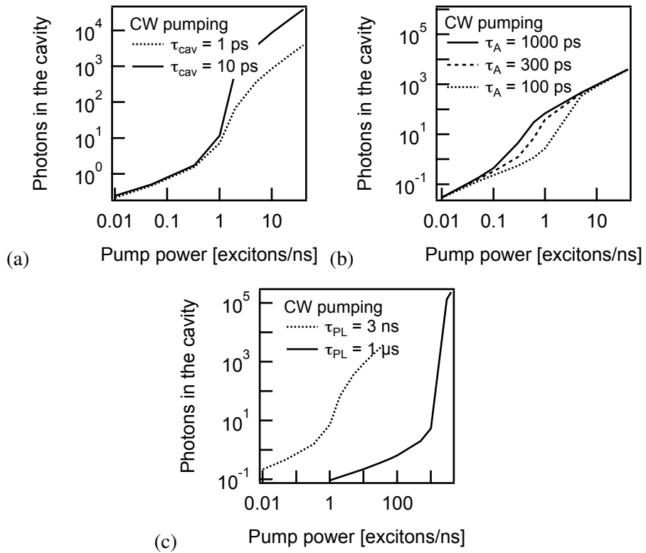
Figure 7.14: Log-log plot of the amount of photons in the cavity as a function of pump power for (a) two different photon cavity lifetimes, (b) three different biexciton lifetimes (note: \beta = 0.5 ), and (c) the spontaneous emission lifetime.
