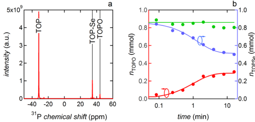
Figure 2.9: (a) ^{31}\text{P} NMR spectrum of the reaction mixture dissolved in toluene- d_8 ( n_{\text{Cd},0} = 0.4 mmol, n_{\text{Se},0} = 1 mmol, 245^\circ\text{C}/230^\circ\text{C} injection/growth temperature, sample taken after 1 min of reaction time) indicating the ^{31}\text{P} resonances of TOP, TOP-Se and TOPO. (b) Time evolution of the concentrations of (red) TOPO, (blue) TOP-Se and (green) their sum. The red and blue full lines are guides to the eye, the full green line indicates the initial amount of TOP-Se in the reaction mixture.
