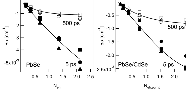
Figure 6.5: Differential absorption as a function of average number of excitons N_{eh} 5ps after the pump pulse (full symbols) and 500 ps after the pump pulse (open symbols) at 1700 nm (triangles), 1850 nm (squares) and 2000 nm (circles) for (a) PbSe QDs and (b) PbSe/CdSe QDs. The full lines are fits to a Poissonian state filling model.
