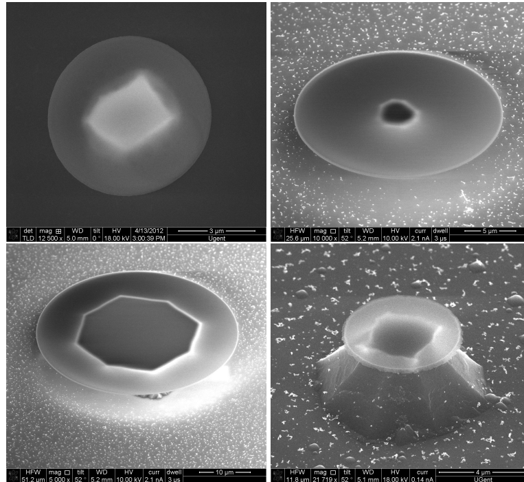
Figure 8.8: Common pillar shapes from KOH wet etching.
