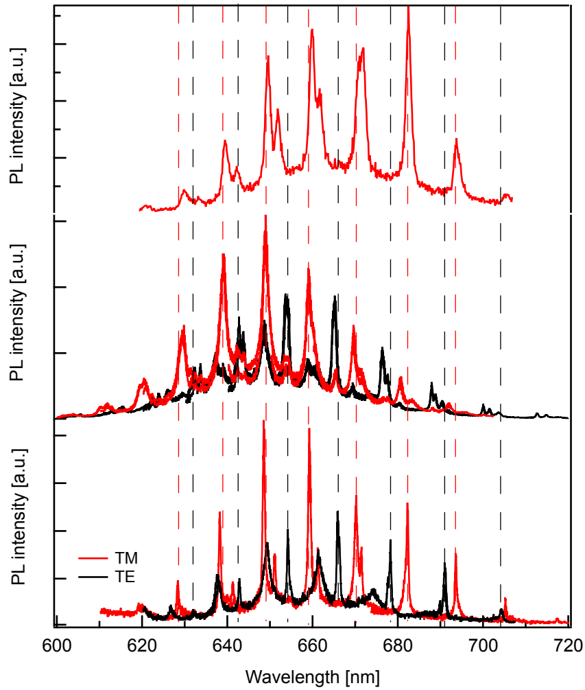
Figure 8.24: TE and TM spectra of three disks of 6.5 \mu\text{m} on the same sample. All disks contain CdSe/CdS dot-in-rods ( 22.3 \text{ nm} by 5.3 \text{ nm} ) and are excited using a 532 \text{ nm} CW laser at low power. Lines are drawn as guides to the eye, showing the corresponding WGMs in each spectrum. The top spectrum was moved by 3.8 \text{ nm} towards the blue (left) side. It illustrates the reproducibility and quality of the microdisks on one sample.
