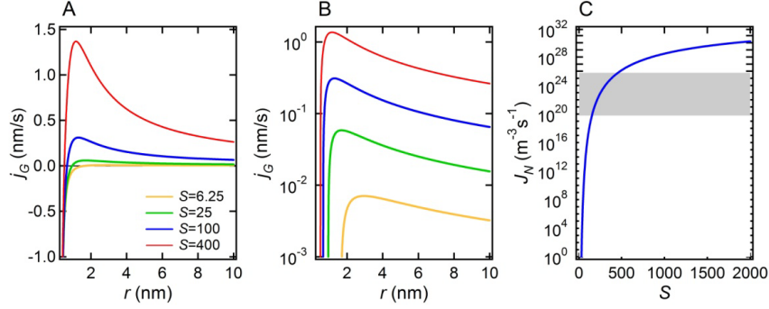
Figure 2.1: (a) Quantum dot growth rate calculated according to eq. 2.4 with the parameters as given in Table 2.1 for different values of the supersaturation S . (b) idem in logarithmic scale. (c) Nucleation rate calculated according to eq. 2.7 with the parameters as given in Table 2.1. The grey region indicates nucleation rates from 0.1 M/s to 0.1 \mu M/s.
