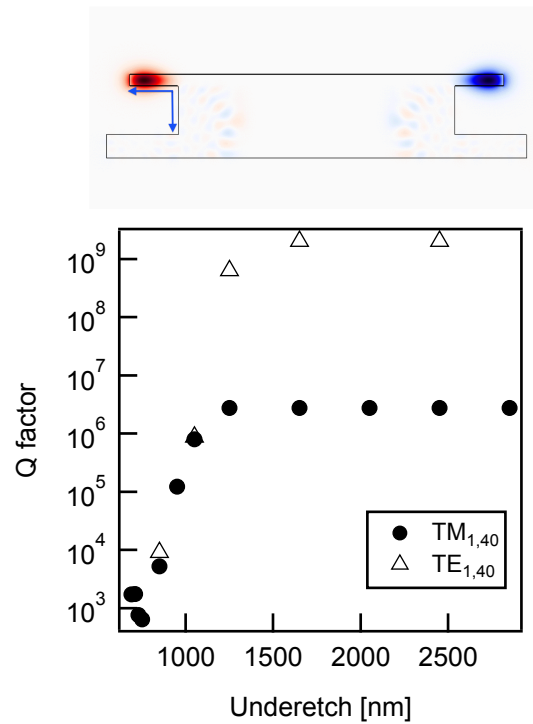
Figure 7.2: Influence of the underetch depth (blue arrows) on the Q factor of the fundamental TE and TM modes shows the radiative loss of the optical mode to the silicon pillar and substrate, when the pillar is not small enough.
