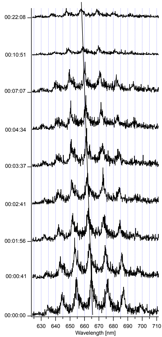
Figure 8.28: Spectra of a 6.5 \mu\text{m} microdisk under 400 \text{ nm} pulsed excitation ( 27 \text{ mW} average power) shifts in time. The time axis increases from the bottom spectrum to the top spectrum.
