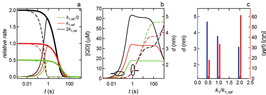
Figure 2.10: (a) (boldlines) Monomer generation rate; (full lines) rate of monomer consumption by growth; (dashed lines) rate of monomer consumption by nucleation for three different values of the first-order rate constant of monomer generation. Red: the value used in Figure 2.2 ( k_1 ). Green: k_1/2 . Black: 2k_1 . (b) (full lines) Change of the QD concentration and (dashed lines) the average QD diameter as a function of time. (c) (blue bars) QD diameter and (red bars) QD concentration at the end of the focusing regime.
