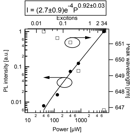
Figure 8.31: Log-log plot of the intensity as a function (left axis, dots) of average power of the fs-pulse laser for the peak wavelength indicated on the right axis with the squares, increases almost linearly. The line is a power law fit to the intensity data as a function of average pump power. The fitting coefficients are given in the box above the graph. The peak wavelength blueshifts over almost the entire FSR for high pump power.
