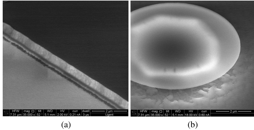
Figure 8.7: (a) RIE of 80 nm of \text{Si}_3\text{N}_4 on top of a silicon substrate using \text{CF}_4:\text{O}_2 30:30 sccm. (b) A finished microdisk shows the smooth edge of the disk when using this gas ratio.
