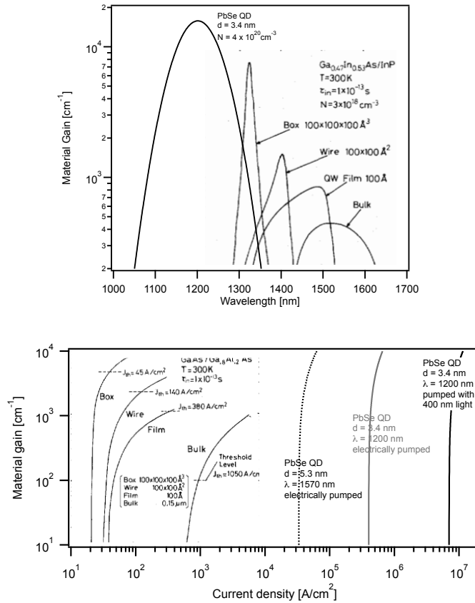
Figure 3.3: (a) Comparison between the gain spectra of PbSe QDs ( d = 3.4 \text{ nm} ) and III-V gain structures (reproduced from Asada et al. 53 ) with different confinement. (b) Maximum material gain as a function of the injection current density. The data for the III-V structures is reproduced from Asada et al. 53 and shows the clear difference with the very high threshold current density needed for PbSe QDs. The current density for 3.4 nm PbSe QDs in black has the meaning of the number of excitons created per second by a 400 nm CW optical pump source (multiplied by e ) per unit area. The grey ( d = 3.4 \text{ nm} ) and the dotted ( d = 5.3 \text{ nm} ) curves plot the material gain vs. the current density for electrical injection.
