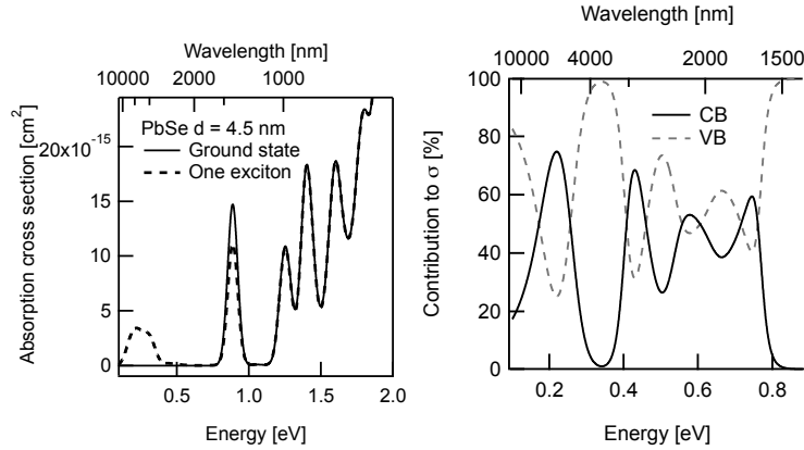
Figure 6.8: (a) Theoretical absorption cross section for a 4.5 nm PbSe QD in the ground state and with a single exciton in the 1S state confirms earlier calculations on PbSe for both band gap AB and mid-infrared PA. (b) The percentage for which initial states in the conduction band (full line) and valence band (dashed line) contribute to the absorption cross section below the band gap shows that valence and conduction band state contribute almost equally in the energy range between 0.4 and 0.8 eV.
