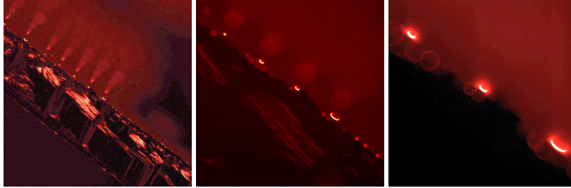
Figure 8.15: Emission imaged with the PL microscope at a 10^\circ angle between the direction of view and the sample plane for increasing magnification from left to right (4x, 10x, 20x)
