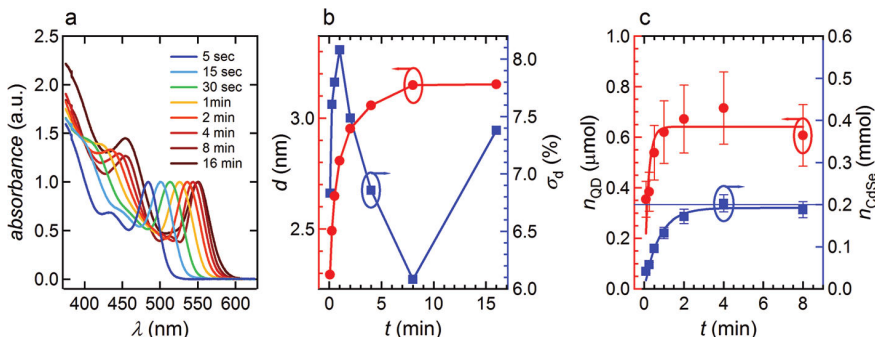
Figure 2.4: (a) Development of the absorption spectrum of CdSe QDs during a standard synthesis ( n_{Cd,0} = 0.2 mmol, n_{Se,0} = 2 mmol, 245^\circ\text{C} / 230^\circ\text{C} injection/growth temperature). (b) Time development of (red circles) the QD diameter d and (blue squares) the size dispersion. (c) Time development of the number of QDs ( n_{QD} , red circles) and the amount of CdSe formed ( n_{CdSe} , blue squares). The full lines are guides to the eye. The horizontal blue line indicates the 100% yield level.
