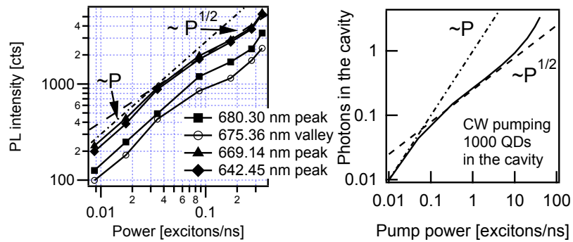
Figure 8.30: (a) Collected PL intensity as a function of CW pump power for several TE modes and one off-mode wavelength shows initially a linear increase, saturating to a square-root dependence. The maximum power indicates a superlinear increase. The dash-dotted line is a guide to eye for a linear dependence, the dashed line indicates a square-root dependence. (b) Simulation of the number of photons in the microdisk cavity as a function of CW pump power, as discussed in Section 7.3.3 (see p. 185) for an underloaded cavity with 1000 QDs shows the same linear increase at low power and sublinear increase at higher power.
