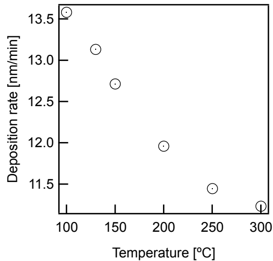
Figure 8.3: The rate of deposition of Si 3 N 4 in PEsCVD for different substrate temperatures.
