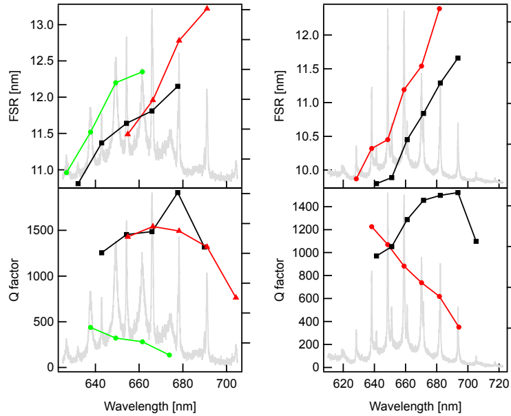
Figure 8.26: FSR and Q factor for the TE (left) and TM modes (right) of a 6.5 \mu\text{m} microdisk.
