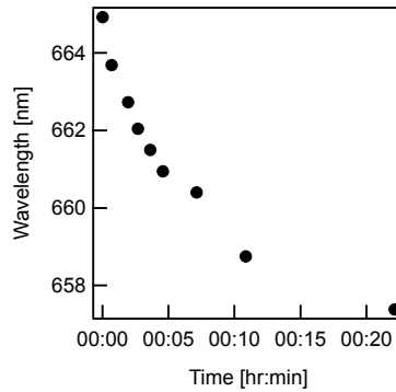
Figure 8.29: Blueshift of one of the WGM peaks as a function of time of excitation using a 400 nm pulsed excitation at full power (27 mW) for a 6.5 \mu\text{m} microdisk.
