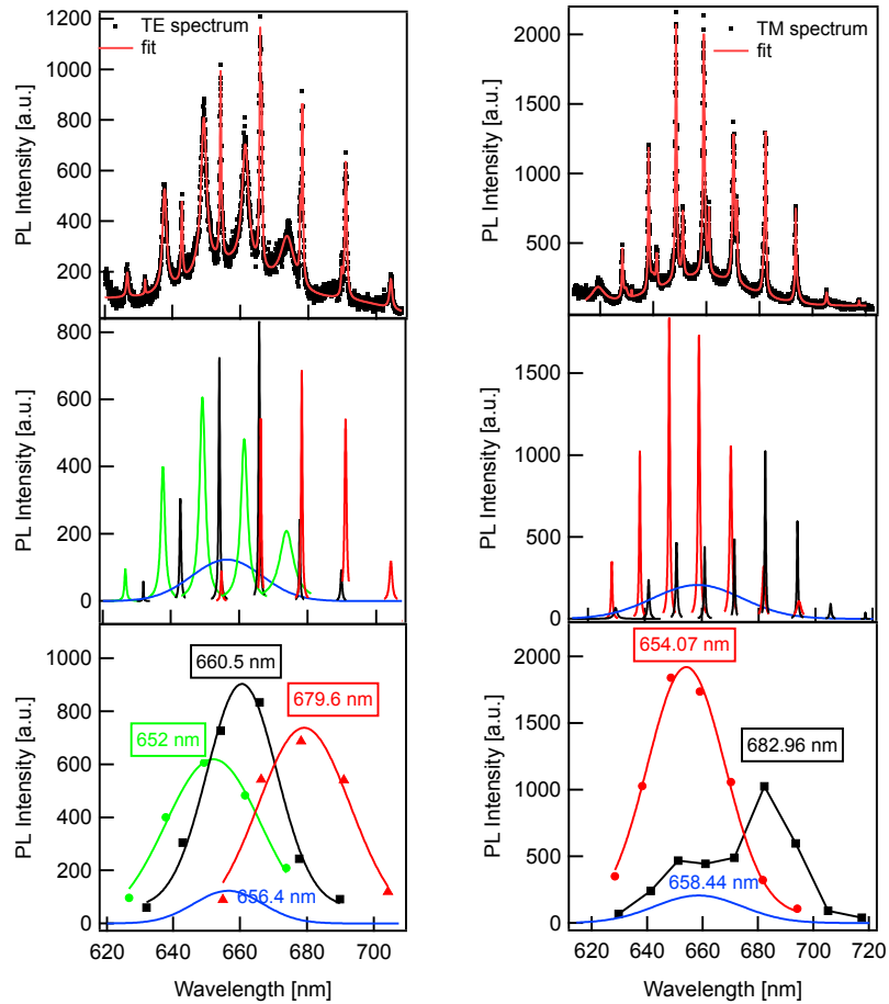
Figure 8.25: (top) The spectrum (TE on the left, TM on the right) of a 6.5 \mu\text{m} microdisk containing CdSe/CdS dot-in-rods is fitted using a multipole fitting algorithm. The sum of all the separate peaks is shown as a red line. (middle) Deconvolution of the spectrum in separate Lorentzian peaks together with a Gaussian background for the uncoupled spontaneous emission. Peaks belonging to the same mode family are coloured in the same way. (bottom) The amplitude of each peak is plotted. The amplitude-envelope of each mode family is fitted using a Gaussian function. The central wavelength is indicated in the boxes.
