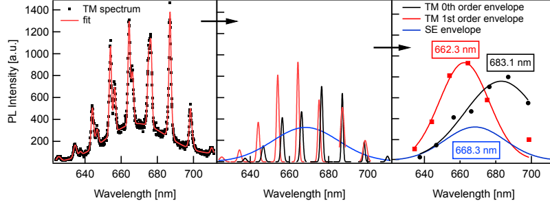
Figure 8.27: Another 6.5 \mu\text{m} microdisk, with similar analysis was done as in Figure 8.25 shows the reproducibility of the processing and measurement.
