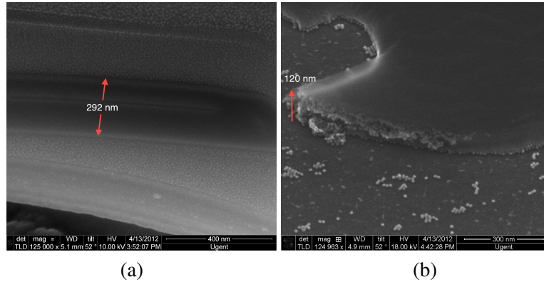
Figure 8.13: (a) Cross section view of a microdisk with 80 nm of low and high index \text{Si}_3\text{N}_4 , and a QD layer, which should have similar height as the layer thickness on the substrate, depicted in (b).
