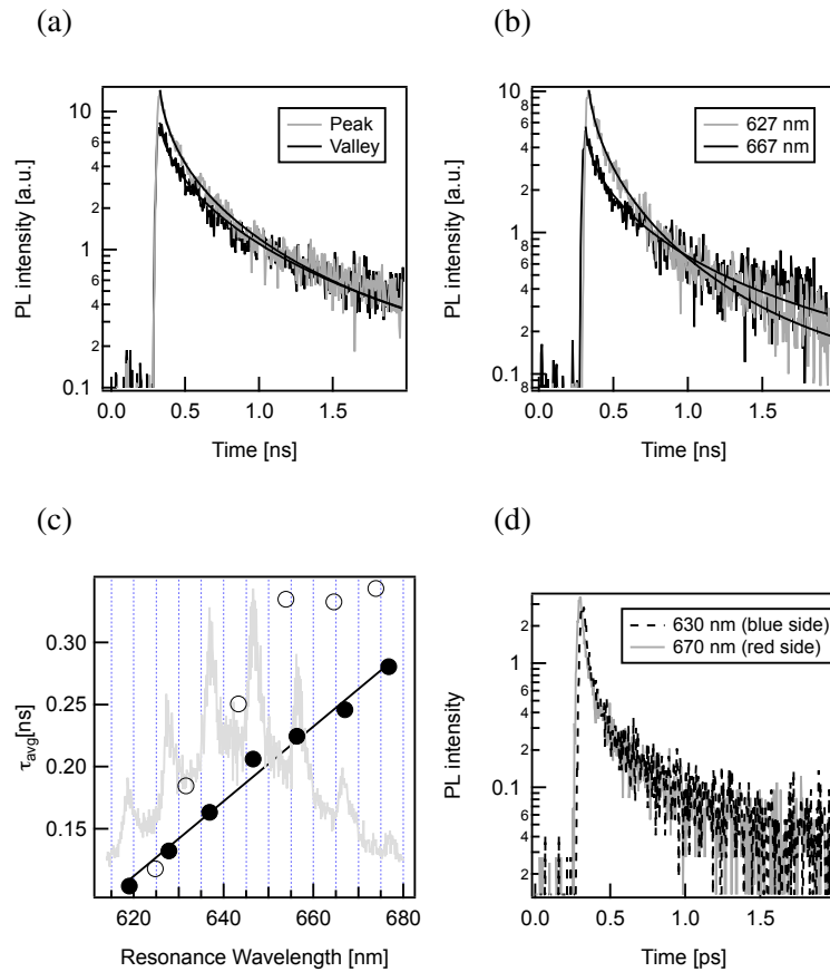
Figure 8.33: (a) The PL decay after excitation with a fs-pulsed laser is shown on resonance (grey) and off resonance (black). The decay curves are fitted using a stretched exponential function. (b) The PL decay after excitation with a fs-pulsed laser is shown at the resonance of 627 nm and 667 nm. We observe a faster decay at the blue side of the spectrum. (c) The average PL decay time for each resonance in the spectrum increases linearly with increasing wavelength (full circles). The decay times off-resonance are also plotted (open circles) and show that decay is enhanced for on-resonance wavelengths. (d) Comparison of the dynamics of the QDs on the sample substrate, i.e. not coupled to the microdisk at the blue and at the red side of the PL spectrum.
