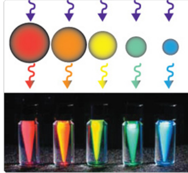
Figure 1.1: Emission colour of a series differently sized CdSe QDs under illumination with a UV lamp shows the effect of quantum confinement.
