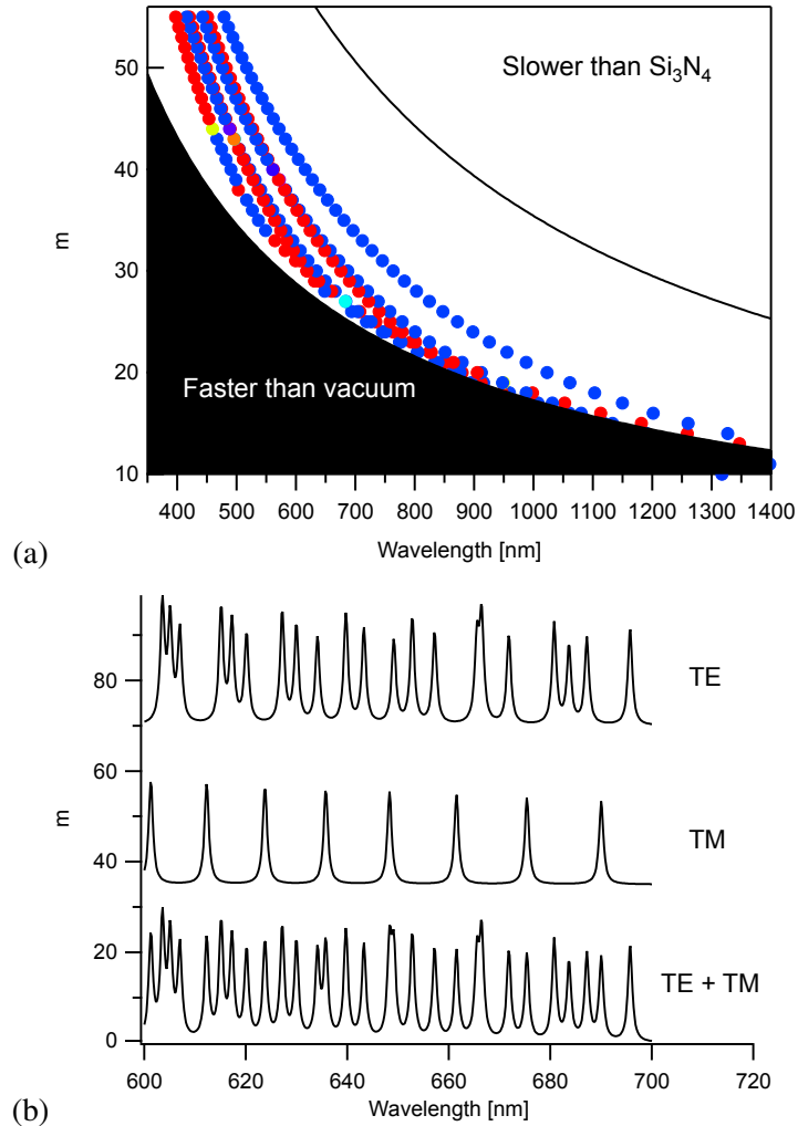
Figure 7.5: (a) Dispersion diagram for a 5.5 \mu\text{m} microdisk depicting the azimuthal mode number m versus the free space wavelength for six modes, as calculated using COMSOL. Blue dots are TE modes, red dots are TM modes. (b) Microdisk emission spectrum, simulated using COMSOL for the TE modes (top), the TM modes (middle) and both polarizations together (bottom). The peaks were artificially broadened with 1 nm FWHM Lorentzian lineshape.
