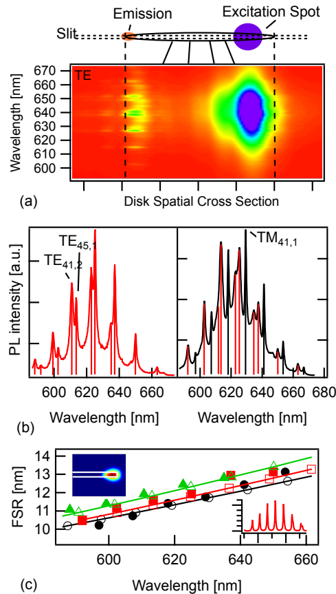
Figure 8.18: (a) Mode map collected from a 6.0\mu\text{m} microdisk containing giant CdSe/14CdS QDs by selective excitation of the right side of the disk. The cross section from where the PL is collected is drawn in the microdisk drawing above. Only TE polarized light is collected here. (b) Spectrum at the left edge of the microdisk for TE and TM polarized light. The two TE modes are also visible in the TM spectrum, as indicated by the red lines.
