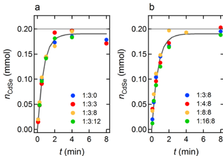
Figure 2.7: Time evolution of the amount of CdSe ( n_{\text{CdSe}} ) for (a) reactions with fixed initial concentrations of Cd(StA) 2 , TOP-Se and StA, and different concentrations of HDA and (b) reactions with fixed initial concentrations of Cd(StA) 2 , TOP-Se and HDA, and different concentrations of StA. The legends give the respective ratios n_{\text{Cd},0}:n_{\text{StA}}:n_{\text{HDA}} . The horizontal lines indicate the 100% yield levels and the full line is a fit through the data points following a mixed second order monomer generation rate model 32 . n_{\text{Cd},0}=0.2 , n_{\text{Se},0}=2 , 245 °C /230 °C injection/growth temperature.
