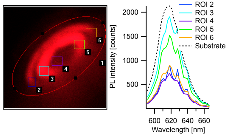
Figure 8.16: (a) Confocal image of a 7 \mu\text{m} microdisk with CdSe/CdS/ZnS QDs at a 10^\circ angle. The Regions of Interest (ROI) are indicated on the image. (b) The spectrum from each of these ROI.
