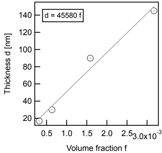
Figure 8.9: Thickness as measured using AFM for a spincoated suspension of QRods (4.5 nm by 22.3 nm) in toluene increases linearly with increasing volume fraction of the QRods.
