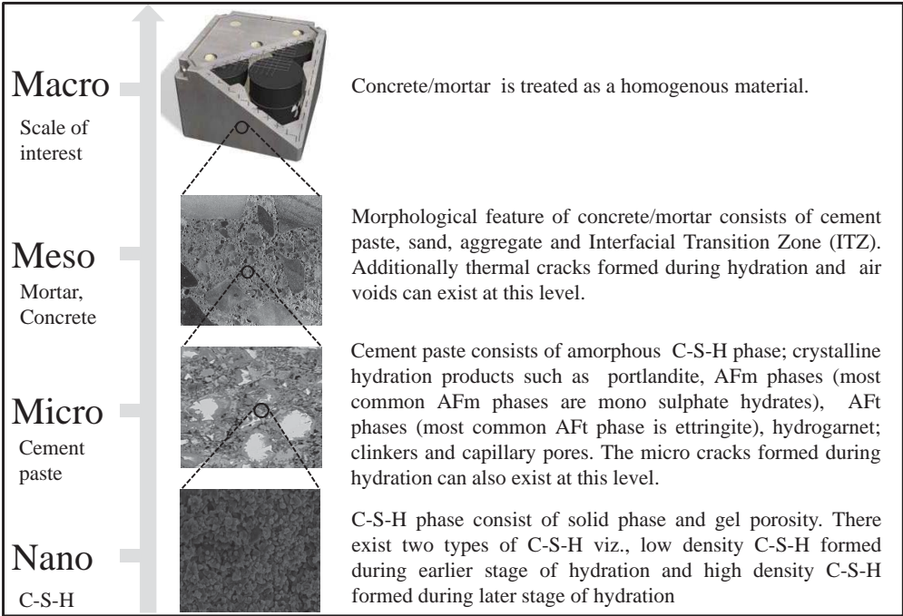
Figure 1.3: Multi-scale representation of concrete
