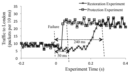
Figure 9: Failure Recovery Experiment Results
