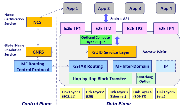
Figure 4: MobilityFirst protocol stack with GUID service layer providing the new narrow waist.
