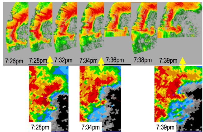
Figure 3: Data from CASA's Oklahoma radar network (top) shows a "hook echo" forming at the center of the image.
