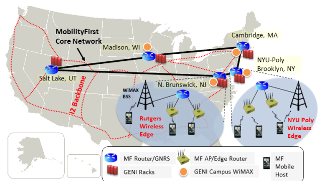
Figure 5: Wide-area deployment of MobilityFirst prototype network on GENI testbed.
