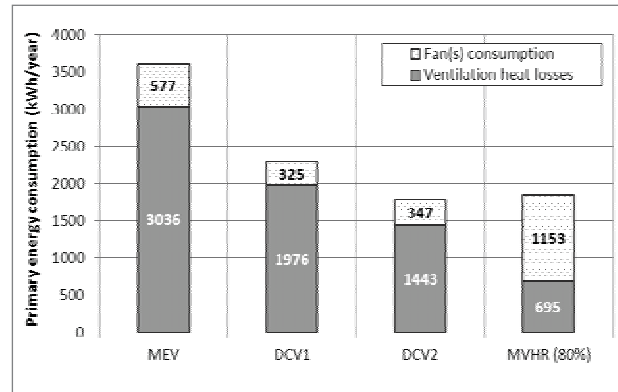
Figure 9: Annual primary energy consumption (kWh/year) of MEV, DCV1, DCV2 and MVHR( \eta = 80\% )
