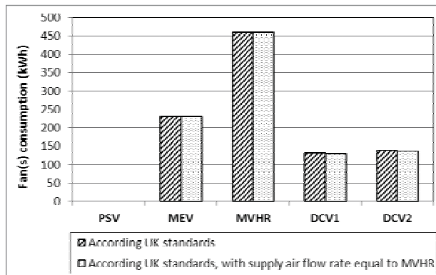
Figure 8: Annual fan(s) electricity consumption for the several mechanical ventilation systems for the location of London at a building air tightness of 3 m 3 /h.m 2 , according to UK standards (left) and with adapted air supply rates (right)
