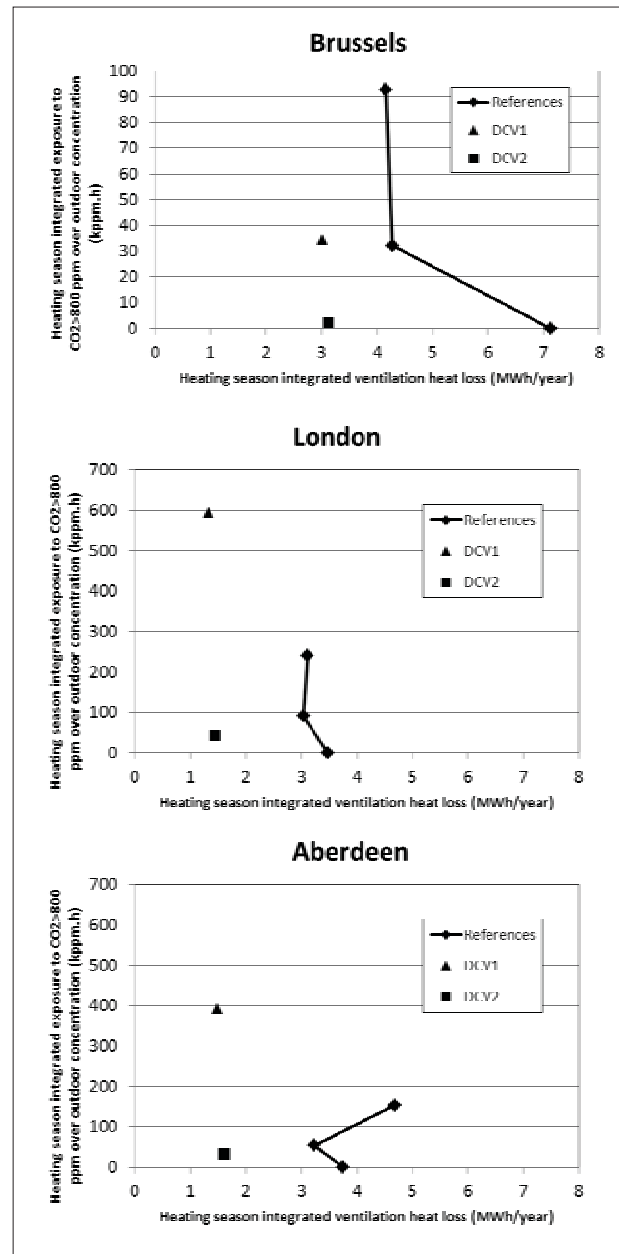
Figure 4: Average cumulative CO_2 concentrations (kppm.h) above 800 ppm over outdoor CO_2 -concentration against ventilation heat loss (MWh/year) for the reference and the DCV1 and DCV2 ventilation systems for the three locations according to current Belgian and British standards
