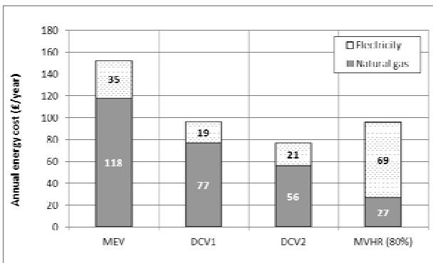
Figure 11: Annual energy costs of MEV, DCV1, DCV2 and MVHR( \eta = 80\% )
