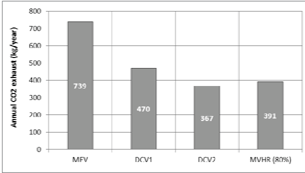
Figure 10: Annual CO 2 exhaust (kg/year) of MEV, DCV1, DCV2 and MVHR( \eta = 80\% )
