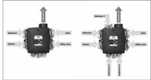
Figure 1: Configuration of DCV 1 (left side) and DCV 2 (right side)
