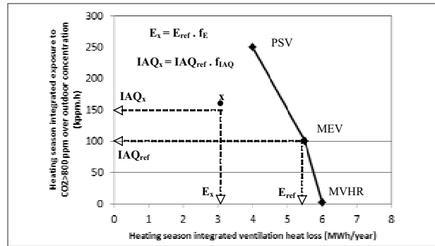
Figure 3: Heating energy and IAQ factor calculation for a ventilation system 'x' with respect to reference systems
