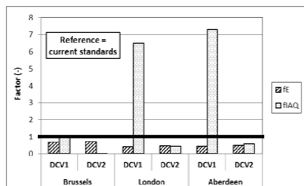
Figure 5: Heating energy ( f_E ) and IAQ factor ( f_{IAQ} ) for DCV1 and DCV2 for the three locations according to current Belgian and British standards
