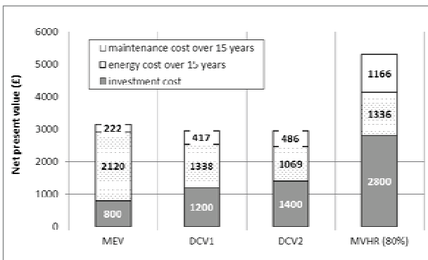
Figure 12: Net present values over 15 years of MEV, DCV1, DCV2 and MVHR( \eta = 80\% )
