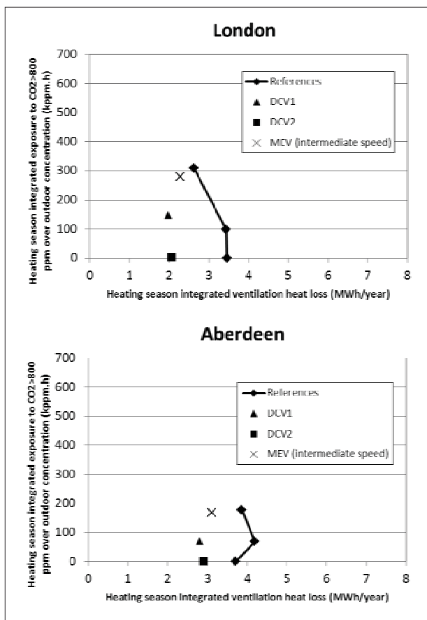
Figure 6: Average cumulative CO 2 concentrations (kppm.h) above 800 ppm over outdoor CO 2 concentration against ventilation heat loss (MWh/year) for the reference and the DCV1 and DCV2 ventilation systems with supply air flow rates equal to MVHR for London and Aberdeen
