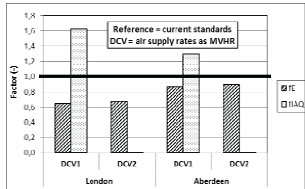
Figure 7: Heating energy ( f_E ) and IAQ ( f_{IAQ} ) factor for DCV1 and DCV2 for London and Aberdeen with adapted DCV air supply rates
