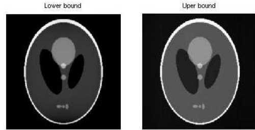
Fig. 5 Lower and upper bounds of the interval-valued representation given by the pixelwise minimum and maximum of the three reconstructed images in Figure 2.
