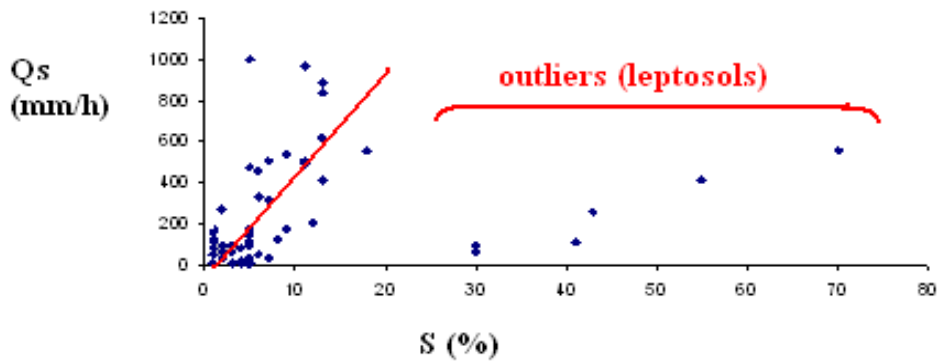
Figure 6. Field-saturated infiltration rates ( Q_s ) as a function of slope gradient ( S ). Values of Q_s are treated as outliers for S > 25\% .
