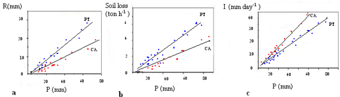
Figure 8. Contrasts between Plain Tillage (in blue) and Conservation Agriculture (in red) for the relations between daily rainfall ( P ) and (a) daily runoff ( R ), (b) soil loss, and (c) infiltrated water ( I ) as measured on the runoff plot. Every dot represents the average of measurements on 3 subplots.
