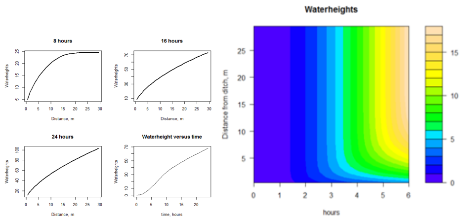
Figure 9. Ponding water height (mm) on CA for runoff lengths (m) and storm duration (hours).
