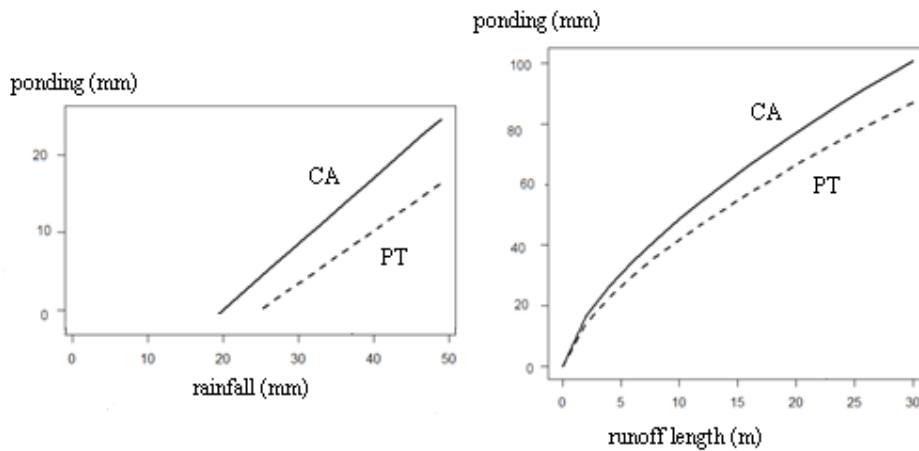
Figure 10. Modelled height of the ponding water (mm) for different rainfall depths, and runoff lengths
