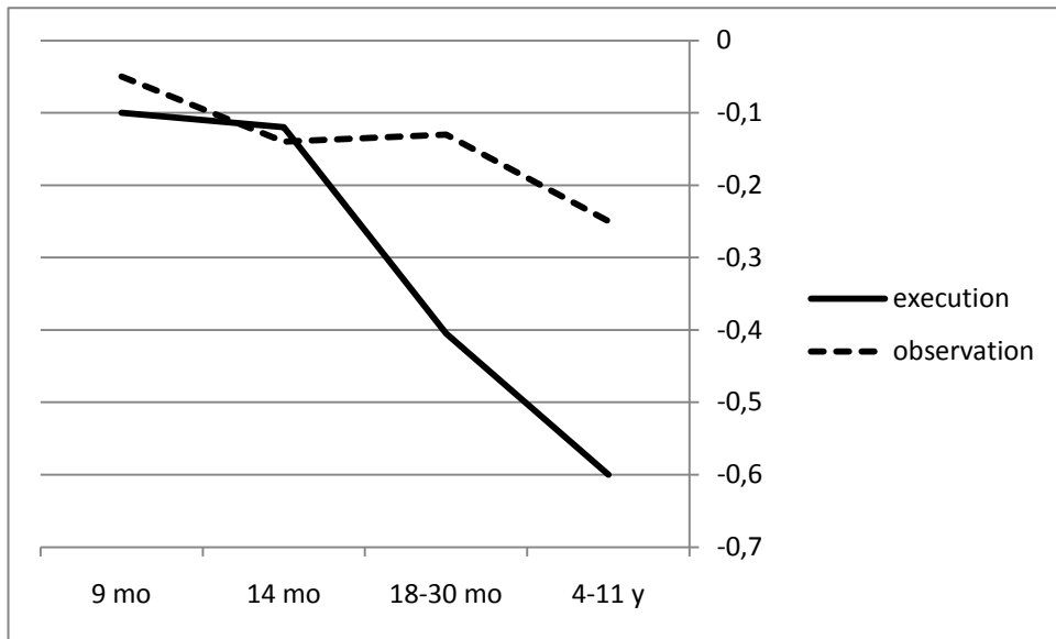
Figure 2. Mu suppression values for action execution and action observation reported by Southgate et al. (2009) in 9-month-olds, by Marshall et al. (2011) in 14-month-olds, found in the current study in 18- to 30-month-olds, and reported by Lepage & Théoret (2006) in 4- to 11-year-olds.
