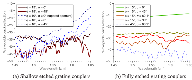
Fig. 5. Reflection spectra for shallow (a) and fully etched (b) grating couplers, each time for different values of the waveguide angle \sigma and fiber tilt angle \phi .
