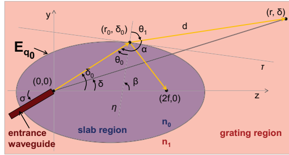
Fig. 1. Focusing grating coupler geometry parameters. The light (yellow arrows) is refracted and reflected at the first grating ellipse E_{q_0} . \tau and \eta are the tangent and normal line respectively of ellipse E_{q_0} at point (r_0, \delta_0) .
