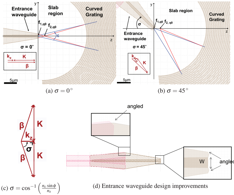
Fig. 2. Reflection from curved grating couplers for different waveguide angles \sigma . The k-diagram is drawn for \sigma = 0^\circ (a), \sigma = 45^\circ (b) and \sigma = \cos^{-1}\left(\frac{n_c \sin \phi}{n_s}\right) (c) which corresponds to both the optimal reflection waveguide angle and second order reflection angle. ( \vec{K} = reciprocal lattice vector) The entrance waveguide is optimized for low reflection (d).
