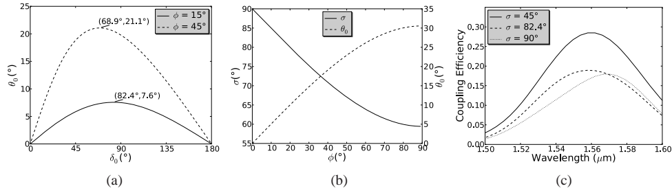
Fig. 3. The reflection angle \theta_0 as a function of \delta_0 for \phi = 15^\circ (a) and the optimal entrance waveguide angle \sigma and corresponding \theta_0 as a function of \phi (b) for \lambda_0 = 1.55 \mu\text{m} . Simulated coupling efficiency (c) for different waveguide angles \sigma (etch of 70 nm, \phi = 15^\circ ).
