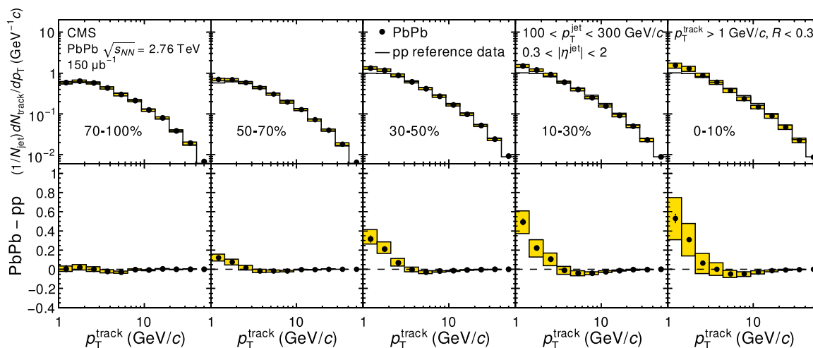
FIG. 5. (Color online) The spectrum of tracks inside the cone of jets with 100 < p_T^{\text{jet}} < 300 GeV/ c , as a function of track p_T , for PbPb (with increasing centrality from left to right) and pp . Both the PbPb and pp results are background subtracted, in the same manner as for the fragmentation function. The bottom panels show the difference of PbPb and pp spectra, demonstrating an excess of low- p_T tracks in the PbPb events.
