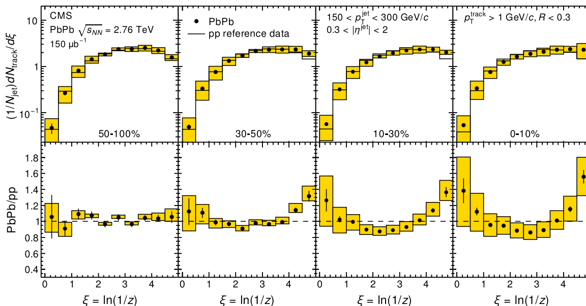
FIG. 4. (Color online) (Top) The PbPb fragmentation function in bins of centrality (increasing from left to right) overlaid with pp reference data. Jets have 150 < p_T < 300 GeV/ c , and tracks have p_T > 1 GeV/ c . (Bottom) The ratio of each PbPb fragmentation function to its pp reference. Error bars are statistical, and boxes show the systematic uncertainty.
