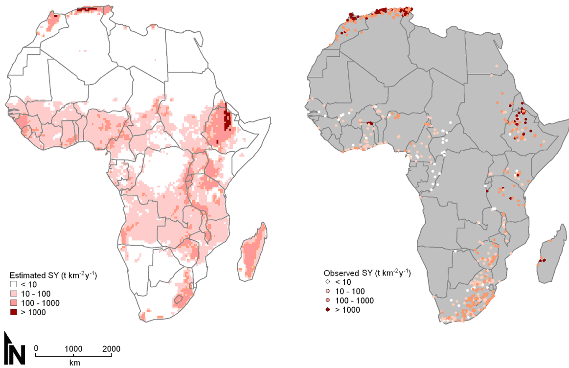
Figure 13: Left: Estimated spatial patterns of sediment yield (SY) in Africa, obtained by applying Eq. 1 to gridded datasets (table 3) and resampling the obtained pixel-values to a 50x50 km 2 resolution. Right: observed catchment sediment yields at their outlet location according to the same classification as the left map for all catchments with available SY observations (n = 682).
