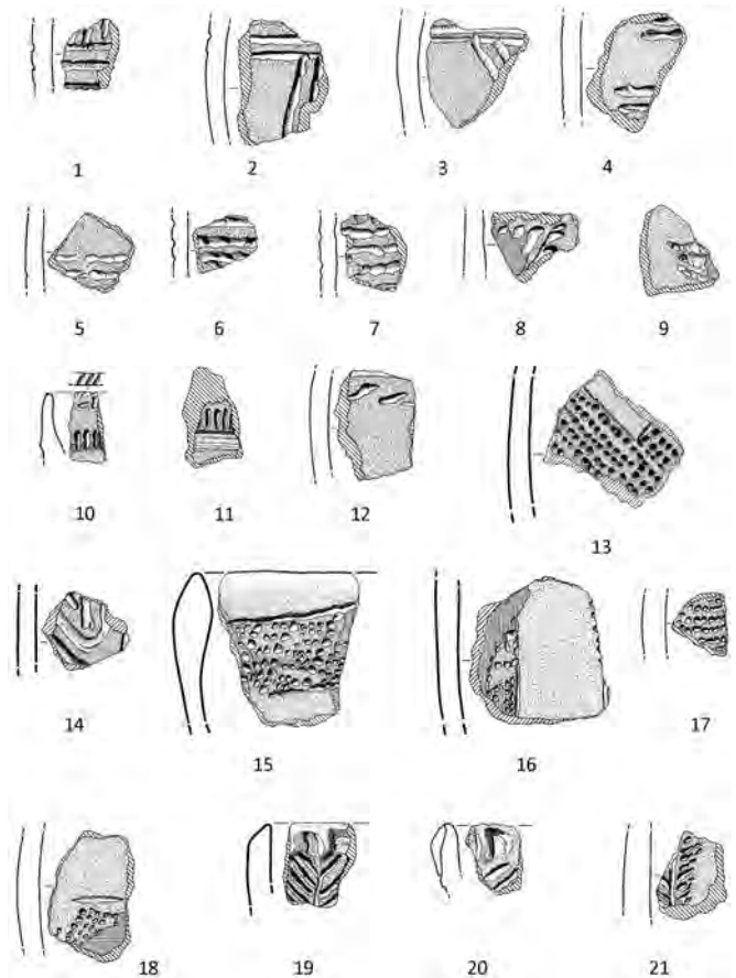
Fig. 7 Bazel (prov. Oost-Vlaanderen/B). Grog and plant tempered pottery. – (Drawings M. Van Meneen). – Scale 1:4.
