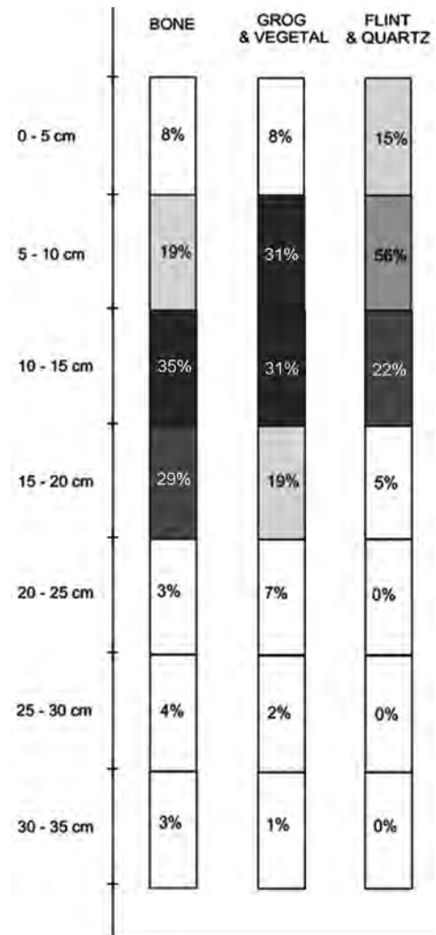
Fig. 11 Bazel (prov. Oost-Vlaanderen/B). Latent stratigraphy based on the vertical distribution of the different pottery groups. – (Illustration J. Sergant).
