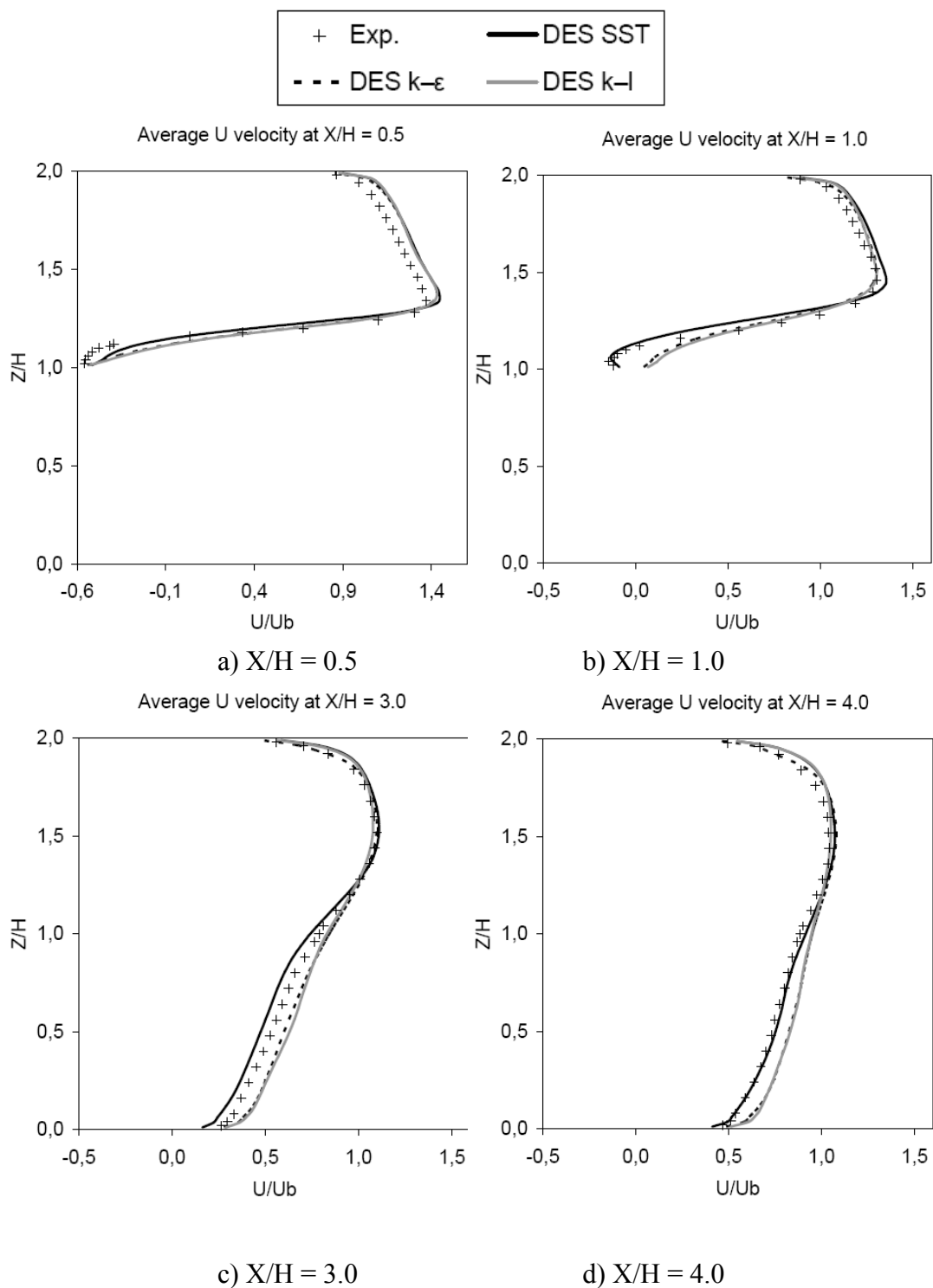
Figure 8: Cube in channel. Mean streamwise velocity in the symmetry plane at X/H = 0.5, 1.0, 3.0 and 4.0 for Hybrid simulations. DES k-\epsilon and DES k-l without wall model. DES SST k-\omega with wall model of Fluent.
