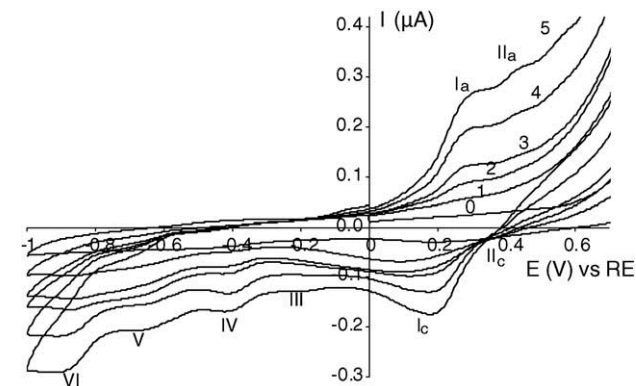
Fig. 4. Cyclic voltammograms recorded at a platinum disc electrode in a methyl methacrylate solution containing 0.1 mol L -1 TBABF 4 and different concentrations of Ru(II)Cl 2 (PPh 3 ) 3 . Concentrations are: (0) 0, (1) 1.48 × 10 -4 , (2) 2.91 × 10 -4 , (3) 4.28 × 10 -4 , (4) 7.49 × 10 -4 and (5) 0.00104 mol L -1 ; T = 298.0 K, \nu = 50 mV s -1 .
