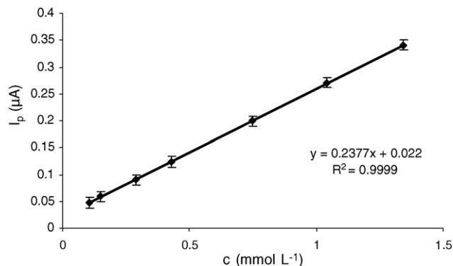
Fig. 5. Calibration plot for the detection of Ru(II) concentrations in 0.1 mol L -1 TBABF 4 methyl methacrylate solution based on the peak current at 0.31 V vs. RE, obtained from cyclic voltammograms shown in Fig. 4; T = 298.0 K, \nu = 50 mV s -1 .
