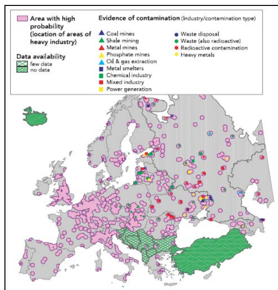
Fig 3. Probable problem areas of local contamination in Europe [2]
