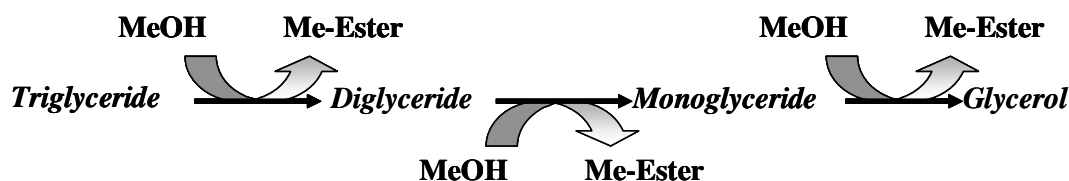
Fig 6. The overall transesterification process of a vegetable oil
