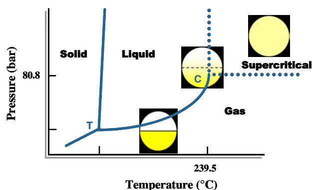
Fig 7. The phase diagram of methanol. The critical point ( T_c = 239.5\text{ }^\circ\text{C} , p_c = 80.8\text{ bar} ) is indicated as "C"
