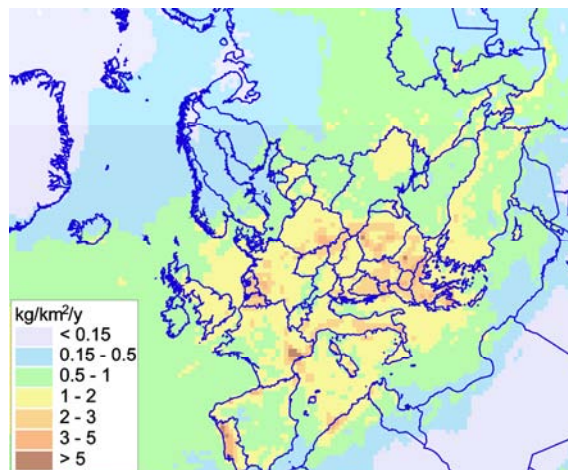
Fig 4. Spatial distribution of lead depositions in Europe in 2004 [3]
