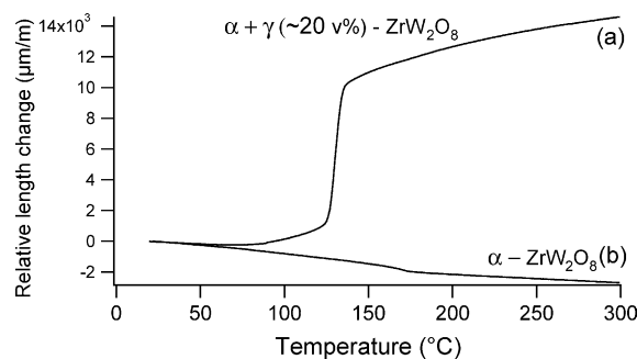
Fig. 4. Thermal expansion curve of (a) a pressed bar containing the α + \gamma -ZrW 2 O 8 mixture and (b) a bar containing pure α-ZrW 2 O 8 . The plot shows the relative change in length from 25 to 300 °C.
