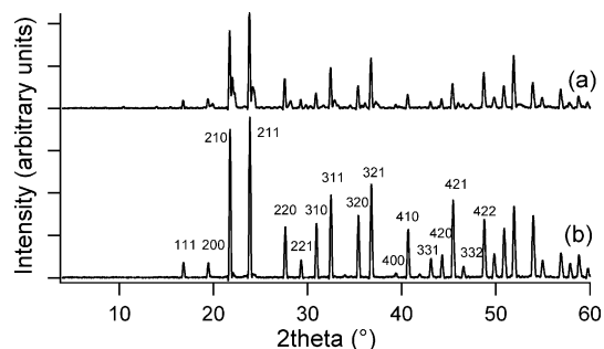
Fig. 3. X-ray diffraction pattern from (a) α + \gamma -ZrW 2 O 8 mixture after pressing, and (b) a pure α-ZrW 2 O 8 phase.
