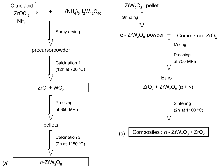
Fig. 1. Synthesis scheme for (a) ZrW 2 O 8 via the spray drying technique and (b) preparation of the ZrW 2 O 8 /ZrO 2 composites.
