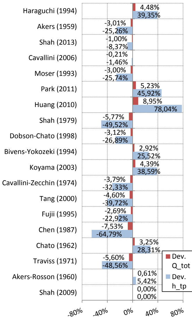
Figure 3 Deviation of Q_{tot} with respect to the deviation of h_{tp}
