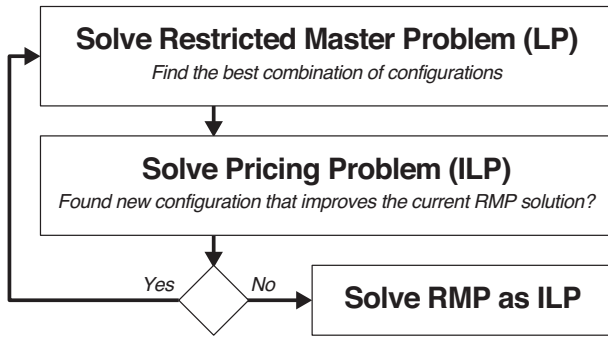
Fig. 2. The general column generation approach.
