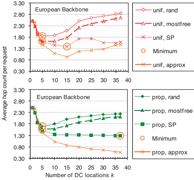
Fig. 1. The required network capacity, which is proportional to the average hop count per request, is minimized by adopting shortest path routing and scheduling (SP), intelligently positioning server capacity ( prop : proportional to the traffic originating closest to that DC), and deploying a reasonable number of server locations. The circled points indicate minimal hop count values per data series. The approx series is the result of analytical approximations and typically underestimates resource requirements.
