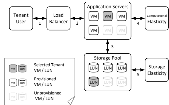
Fig. 2. General overview of a scalable system for data-intensive multi-tenant cloud applications.
