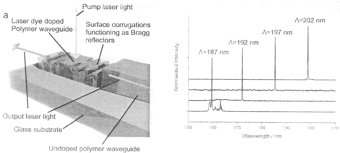
Figure 2: Schematic of polymer DFB-Laser fabricated by combined nanoimprint and photolithography (CNP) and measurement of change in output wavelength of DFB-laser in dependency of the imprinted grating period
