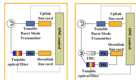
Fig. 2: Architecture of ONU a (left) and ONU b (right)
