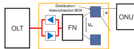
Fig. 1: General hybrid WDM/TDM PON architecture
