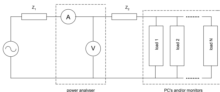
Fig.1. Measurement set-up
