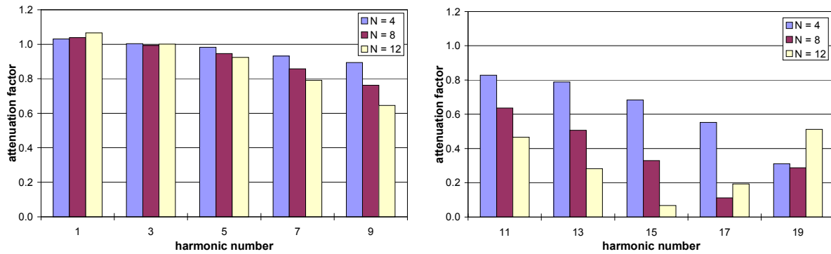
Fig.5. Attenuation factors of harmonic currents
