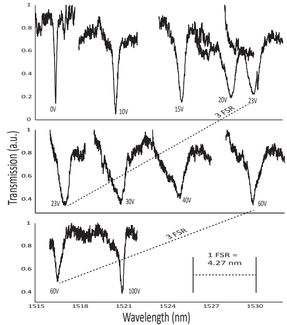
Fig. 3. Output spectrum for different values of the voltage.
