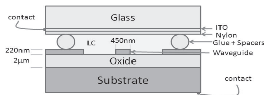
Fig. 1. Schematic overview of a liquid crystal cell.
