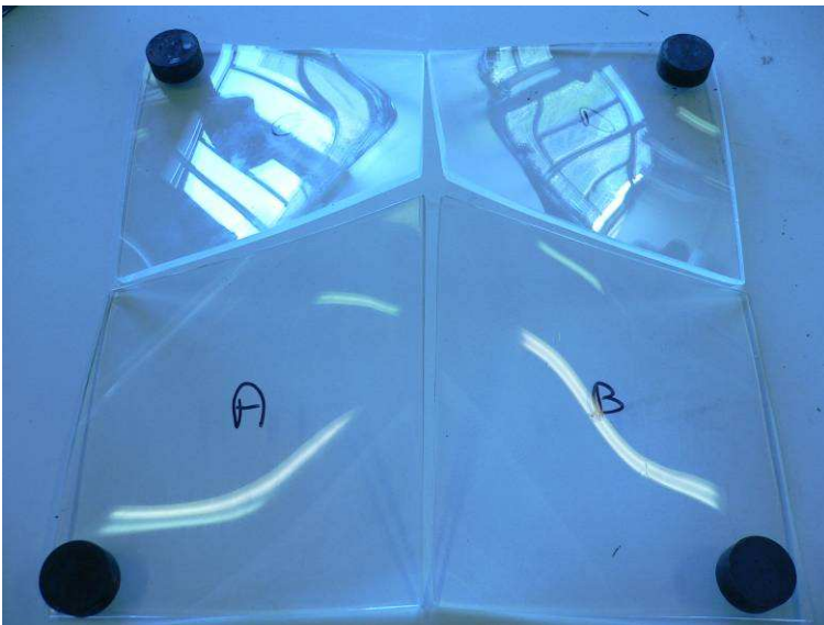
Figure 9: Sample with direct fused glass plates (i.e. without joint filler) on perpendicularly polished edges
