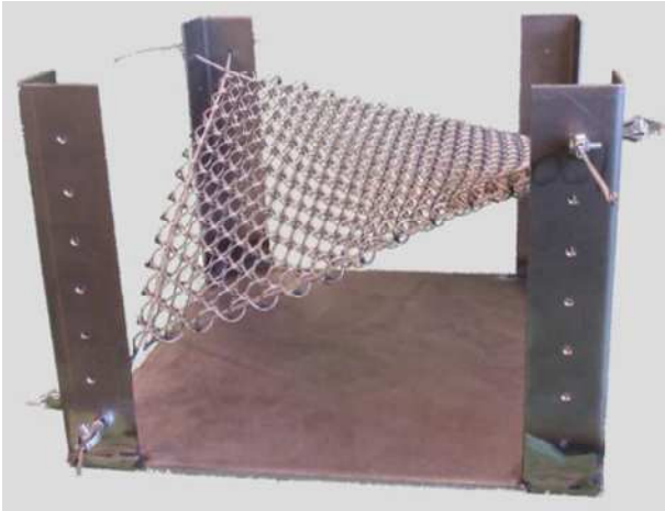
Figure 4: Open stainless steel mesh “Sierra papa 2”. Top: attached to a frame with adjustable plungers (in the oven); Bottom: attached at variable height to steel columns
