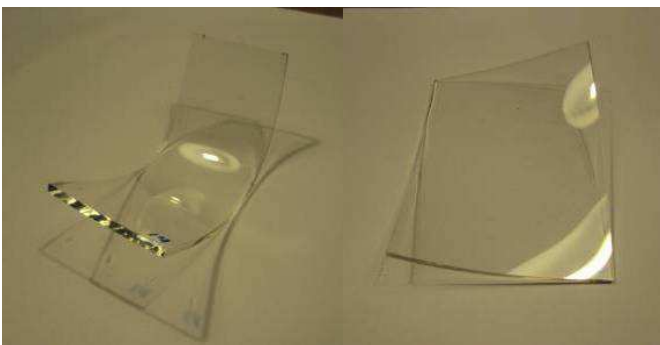
Figure 2: Typical results of preliminary tests: small-scale single and double curved glass shells
