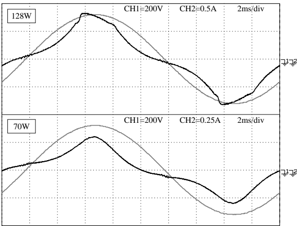
Fig. 13. Input current and input voltage waveforms for 128 and 70W programmed input power, without sample correction and duty-ratio feedforward
