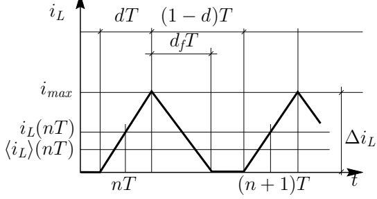
Fig. 4. Input current in DCM
