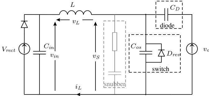
Fig. 5. Parasitic network causing oscillations in the input current, gray: snubber
