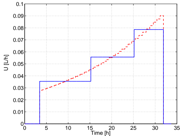
Fig. 2. Optimal and suboptimal feeding rate profile for growth parameter identification.
