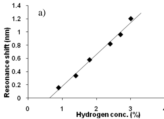
Fig 2 Ring resonator resonance shift measured as a function of hydrogen gas concentration
