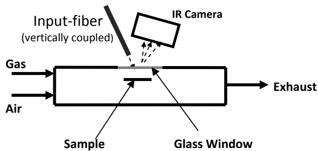
Fig 1 measurement setup
