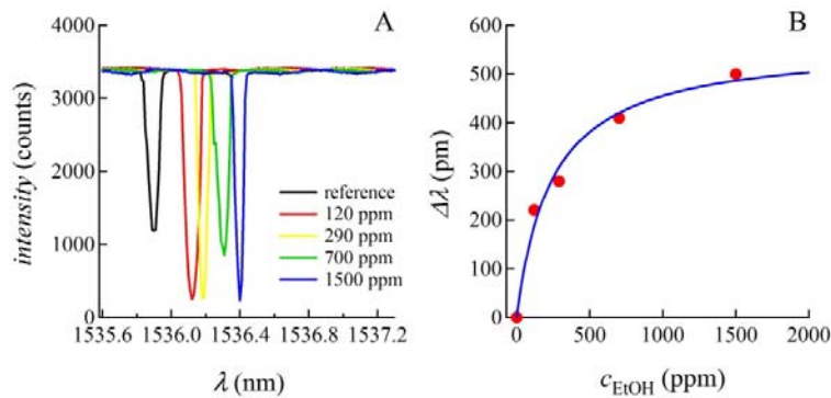
Fig 3 resonance shift measured from a through port of a ZnO nanoparticle film coated MRR at different ethanol vapor concentrations
