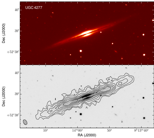
Fig. 5. Top : false colour TNG V -band image of UGC 4277 from Bianchi (2007). Bottom : HI contours overlaid on the same V -band image. Contours start at 3.61 \times 10^{20} \text{atoms cm}^{-2} and increase as 2, 4, 6, 8, and 10 times this value. North is up, east to the left.
