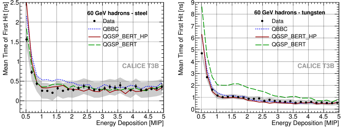
Figure 8. Comparison of the energy dependence of the mean time of first hit of Monte Carlo and test beam data for hadrons in steel (left) and tungsten (right) absorbers. The grey band shows the systematic uncertainties.
