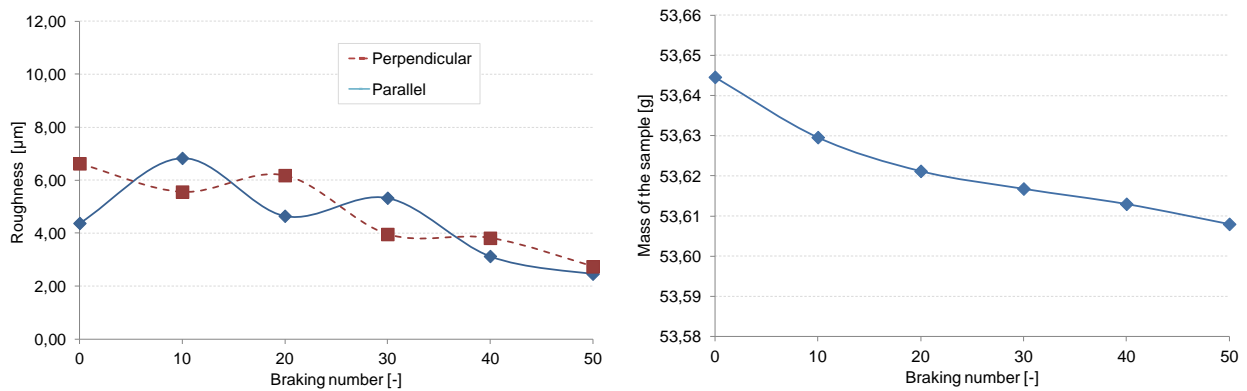
Figure 8. Roughness (left) and wear (right) evolution of the friction material.
