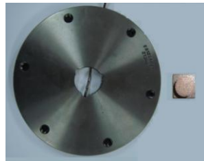
Figure 2. A brake disc (dia.=159 mm) and a brake material sample used in the braking tests.
