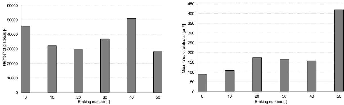
Figure 6. Evolution in number (left) and mean area of the contact plateaus (right).
