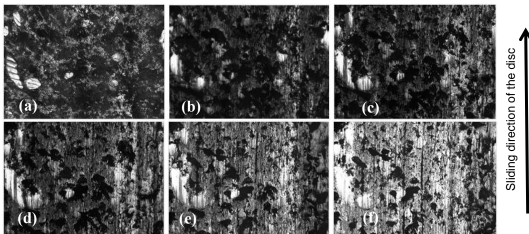
Figure 7. Micrographs of the (a) unused material and after braking number (b) 10, (c) 20, (d) 30, (e) 40, (f) 50.
