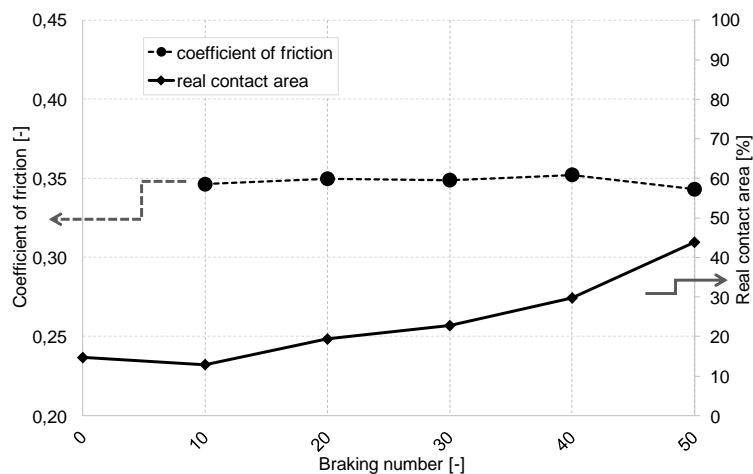
Figure 5. Evolution in friction and real contact area versus braking operation.
