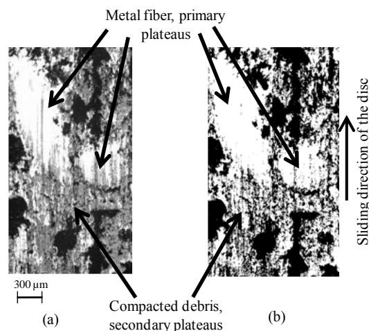
Figure 4. Micrograph of the NAO material: (a) before and (b) after segmentation technique..
