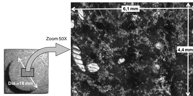
Figure 3. Illustration of a friction material sample and its corresponding area analyzed in the microscope.
