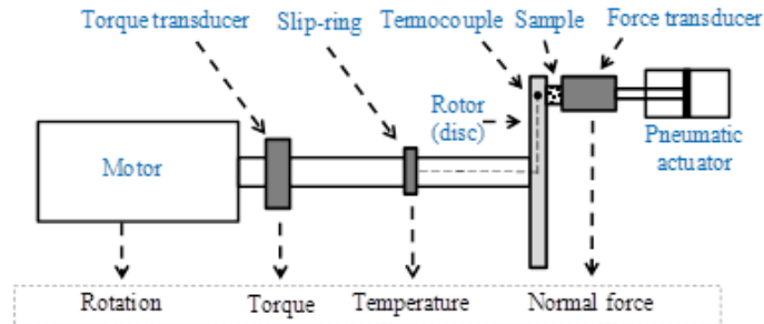
Figure 1. Scheme of the laboratory-scale tribometer.
