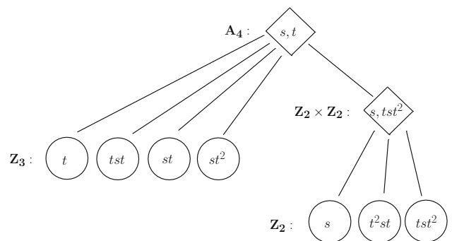
Fig. 2 Diagram of the subgroups of A_4 and their generators, based on Ref. [27]. Invariant subgroups are enclosed in diamond shaped boxes; others are in circles
