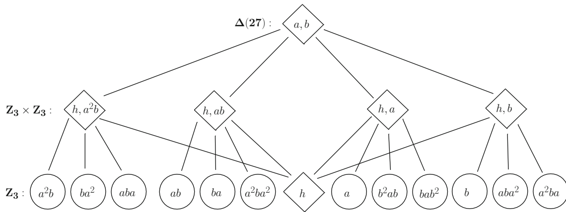
Fig. 1 Diagram of the subgroups of \Delta(27) and their generators, based on Ref. [27]. Invariant subgroups are enclosed in diamond shaped boxes; others are in circles
