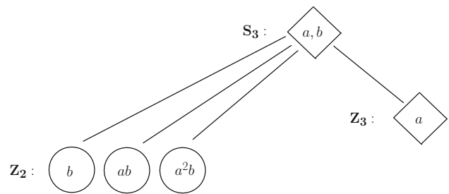
Fig. 3 Diagram of the subgroups of S_3 and their generators, based on Ref. [27]. Invariant subgroups are encased in diamond shaped boxes; others are in circles
