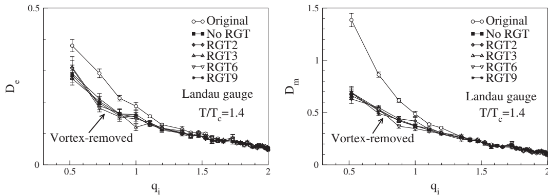
FIG. 3. The dependence of the electric (left panel) and magnetic (right panel) gluon propagators on the Gribov copy ambiguities. The lattice size is 24^3 \times 4 and T/T_c = 1.4 . The RGT with different random seeds is applied to each lattice configuration a varying number of times.
