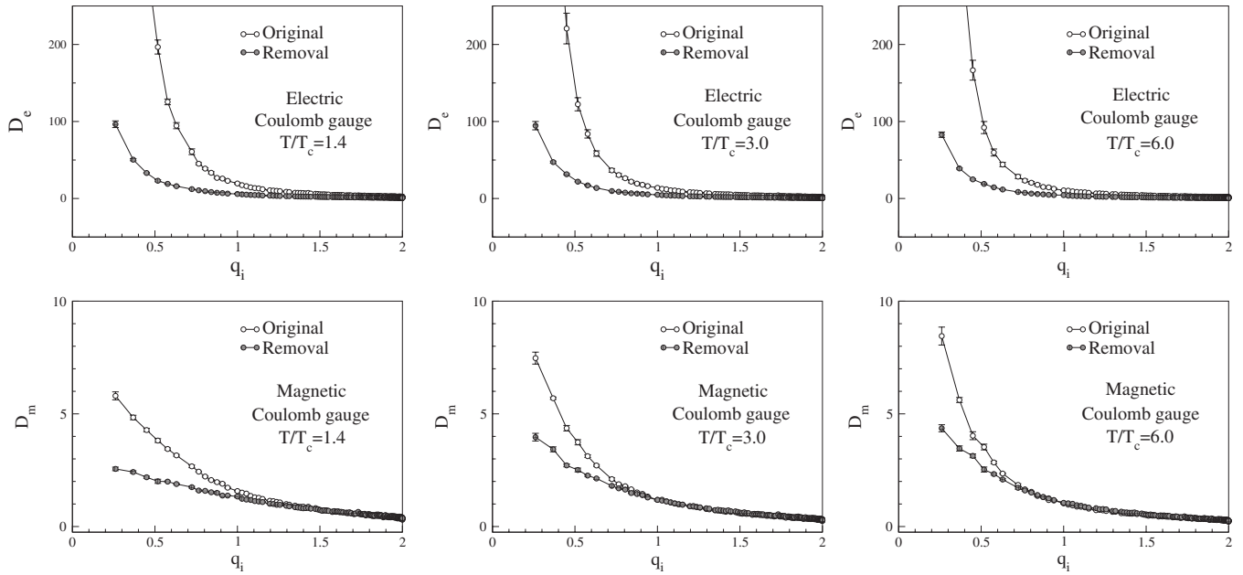
FIG. 2. Electric (upper figures) and magnetic (lower figures) gluon propagators in the Coulomb gauge as a function of the spatial momentum at T/T_c = 1.4, 3.0, and 6.0 . The open symbols represent the numerical results obtained with the use of the original lattice configurations, while the filled symbols correspond to the vortex-removed configurations.
