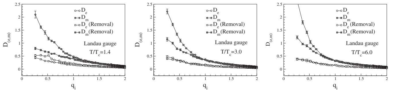
FIG. 1. Electric and magnetic gluon propagators in the Landau gauge for T/T_c = 1.4, 3.0 , and 6.0 as a function of the spatial momentum. The circle symbols represent numerical results obtained with the original lattice configurations, while the square symbols correspond to the vortex-removed configurations.
