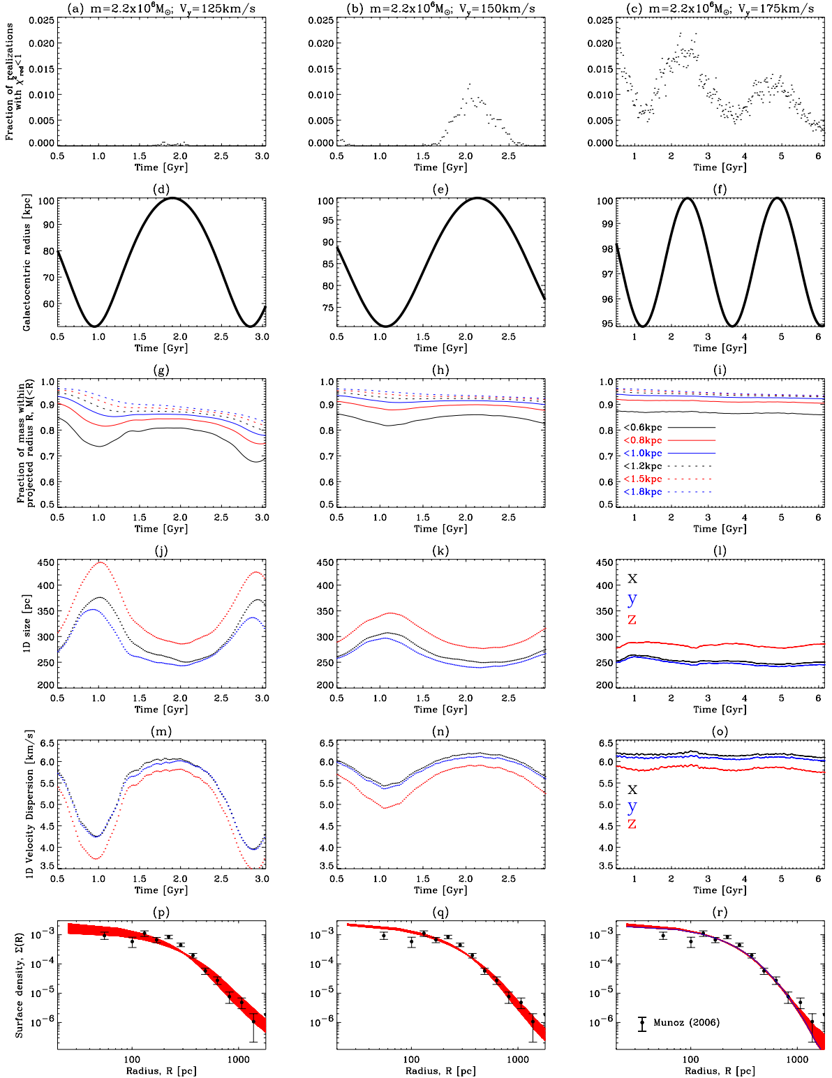
Figure 7. Here we plot six different quantities (each row) for a different orbit (each column) using the same initial conditions and the same initial dSph mass (here m = 2.2 \times 10^6 M_{\odot} ). The three different orbits are defined by their initial tangential velocity ( V_y ) which is in the direction perpendicular to the initial separation between the dSph and the MW of 100 kpc: from left to right V_y = 125, 150 and 175 \text{ km s}^{-1} . (i) The Galactocentric distance as a function of time is the second row of plots and (ii) the top row shows the fraction of random realizations of the projected velocity dispersion which, when compared with the observed one, yield \chi_{\text{red}}^2 < 1 as a function of time. (iii) The third row gives the fraction of projected mass within radial shells of 0.6, 0.8, 1.0, 1.2, 1.5 and 1.8 kpc as a function of time. (iv) The fourth row give the 1D rms size in each of the three directions ( x, y and z ; where z is the line of sight) and (v) gives the 1D rms velocity. (vi) The final row shows surface density profiles (red lines) for evenly spaced snapshots in time. The normalization is the same for every snapshot. The blue line in panel (r) is the initial surface density profiles (red lines) for evenly spaced snapshots in time. Also overplotted (filled circles with error bars) is the observed surface density of stars from Muñoz et al. (2006).
