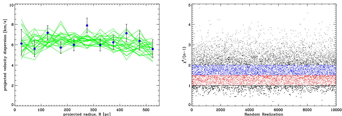
Figure 6. In the left-hand panel, we plot our re-binning of the projected velocity dispersion data from Walker et al. (2007) with blue filled circles. Overplotted with green lines are 25 random realizations of our best-fitting static model of Carina as explained in Section 4. In the right-hand panel, we plot the \chi^2_{\text{red}} distribution of 10k random realizations of the same model. \chi^2_{\text{red}} levels are highlighted with different colours in order to clearly see the number of fits within the ranges \chi^2_{\text{red}} < 1 (large black dots), 1 < \chi^2_{\text{red}} < 1.5 (red dots), 1.5 < \chi^2_{\text{red}} < 2 (blue dots) and \chi^2_{\text{red}} > 2 (small black dots).
