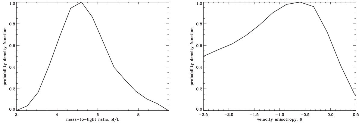
Figure 2. Here we plot the normalized probability distributions of the MOND stellar mass-to-light ratio (left-hand panel) and velocity anisotropy, \beta (right-hand panel) from a Jeans modelling MCMC analysis of the projected velocity dispersions measured by Walker et al. (2007).
