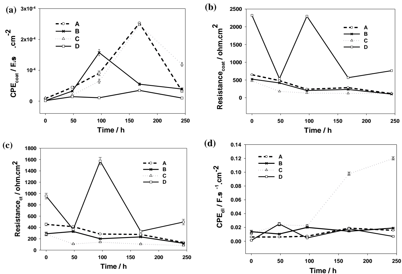
Figure 6. Evolution of the coating capacitance (a); coating resistance (b); charge transfer resistance (c); and double layer capacitance (d) during immersion in a 3.5 % NaCl solution.
