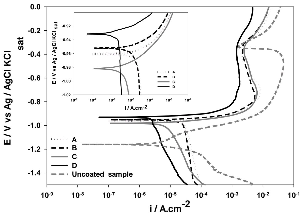
Figure 3. Potentiodynamic polarization curves for the uncoated and coated electro-galvanized steel samples with silane coatings A, B, C and D, obtained after 1 h of immersion in a 3.5 % NaCl solution. The inset shows a zoom around the corrosion potential of the coated samples.
