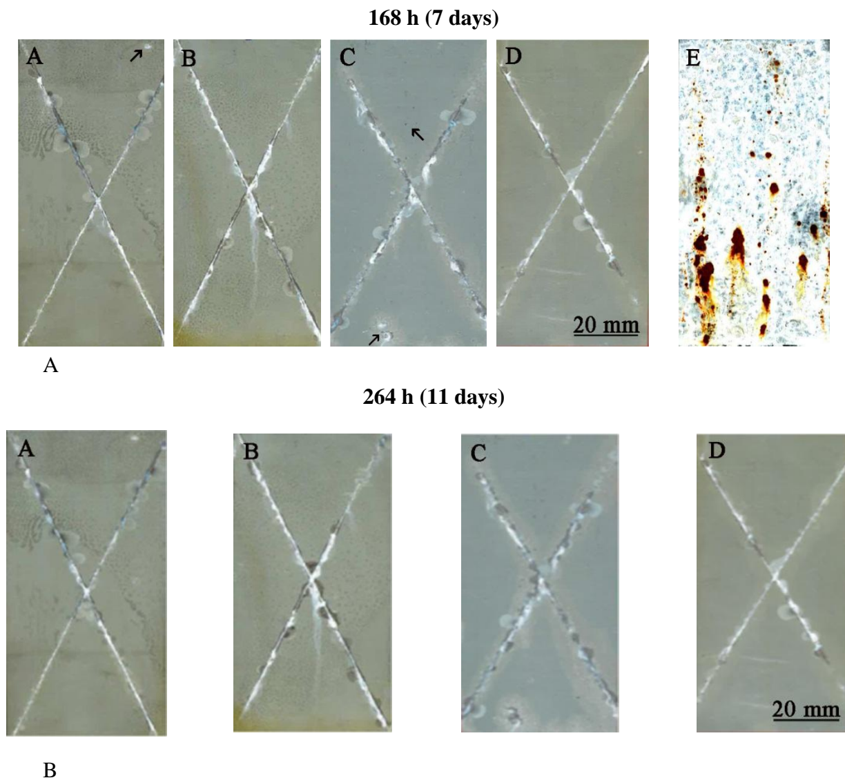
Figure 2. Photographs of uncoated and coated electro-galvanized steel samples with silane coatings A, B, C and D after 168 h (a) and 264 h (b) of salt spray exposure.
