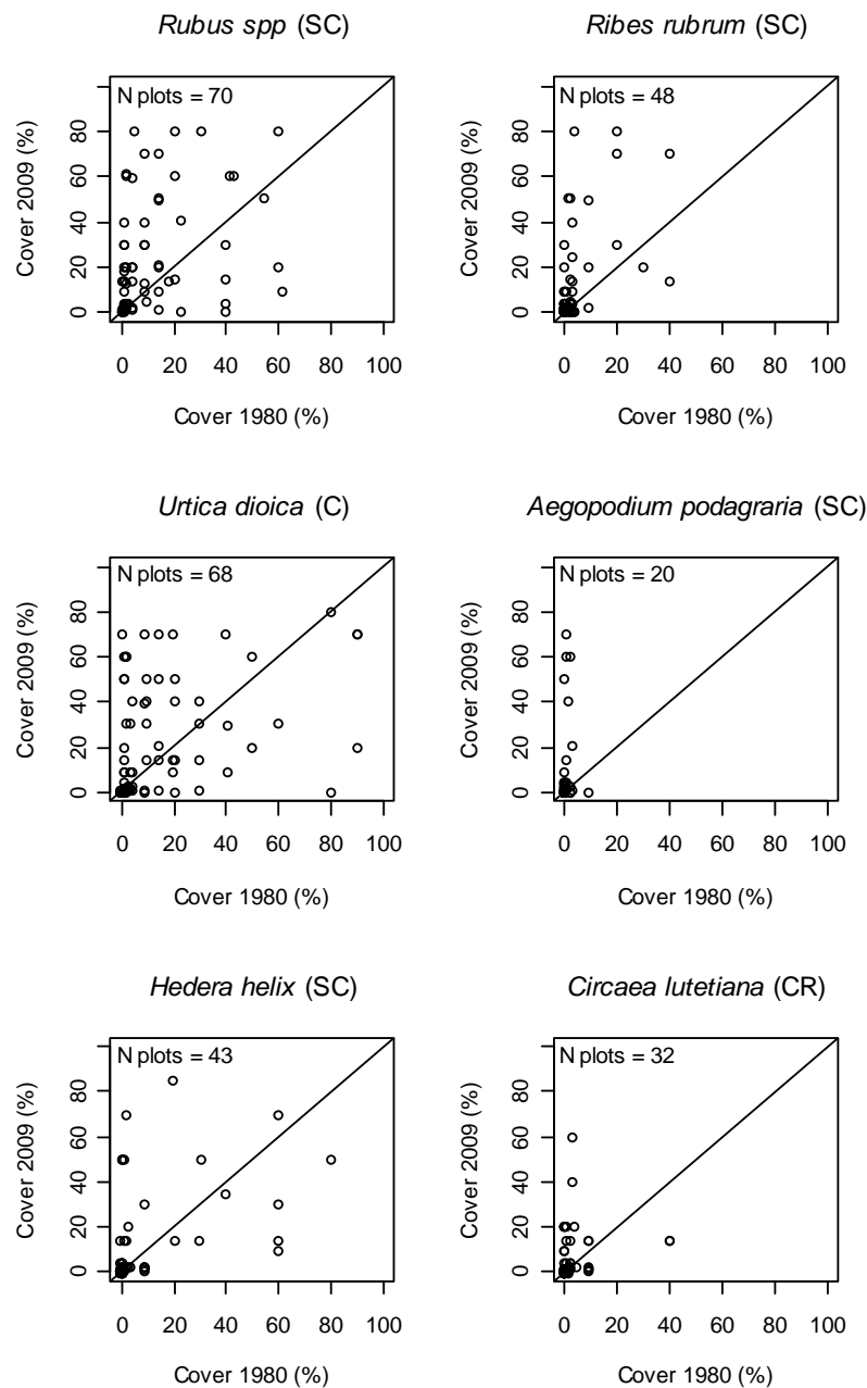
Figure S1 Plot-level changes in species cover (%) for a selection of six species that showed the largest mean absolute change in plot-level cover between 1980 and 2009. The strategy of the species is reported within parenthesis (Hodgson et al. 1995). The “N plots” gives the total number of plots in which the species occurred (total number = 78) in at least one of the two survey years (1980 or 2009).
