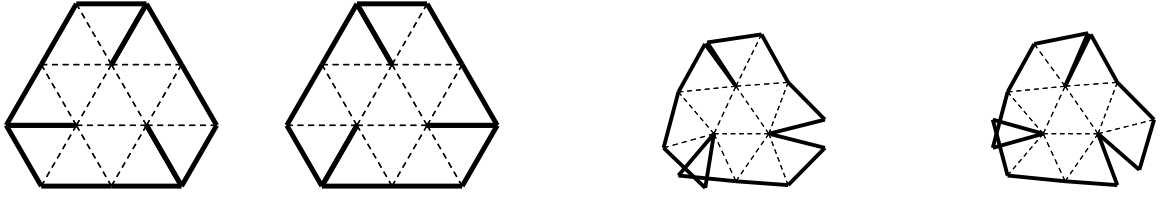
Figure 28 Pair 13 6 . Sunada triple G = \mathbf{PSL}(3,3) , G_i = \langle a_i, b_i, c_i \rangle , i = 1, 2 , with a_1 = (0\ 2)(1\ 7)(3\ 6)(5\ 10) , b_1 = (0\ 6)(2\ 4)(3\ 8)(5\ 9) , c_1 = (0\ 5)(1\ 2)(6\ 12)(9\ 11) , a_2 = (0\ 7)(3\ 11)(6\ 8)(9\ 12) , b_2 = (0\ 8)(1\ 10)(5\ 11)(7\ 9) , c_2 = (0\ 11)(1\ 8)(2\ 7)(3\ 4) .
