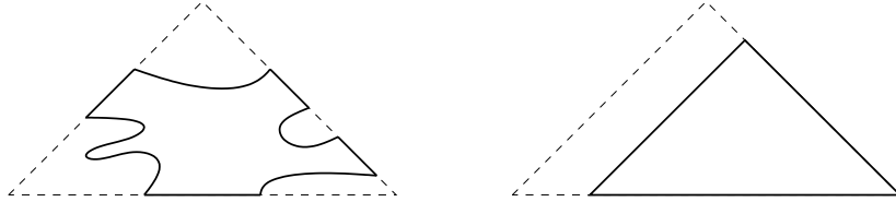
Figure 6 Examples of building blocks yielding isospectral pairs.
