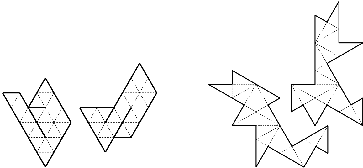
Figure 36 Pair 21_1 . Sunada triple G = \mathbf{PSL}(3,4) , G_i = \langle a_i, b_i, c_i \rangle , i = 1, 2 , with a_1 = (2\ 7)(3\ 11)(5\ 12)(8\ 18)(13\ 14)(15\ 17)(16\ 20) , b_1 = (0\ 17)(3\ 8)(4\ 12)(6\ 13)(9\ 19)(14\ 15)(16\ 18) , c_1 = (1\ 8)(2\ 16)(4\ 11)(5\ 19)(7\ 14)(10\ 17)(13\ 20) , a_2 = (0\ 1)(4\ 17)(7\ 12)(9\ 16)(10\ 20)(11\ 13)(15\ 19) , b_2 = (0\ 20)(3\ 16)(6\ 11)(8\ 15)(9\ 19)(10\ 12)(14\ 18) , c_2 = (1\ 8)(2\ 16)(4\ 11)(5\ 19)(7\ 14)(10\ 17)(13\ 20) .
