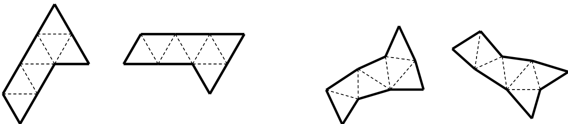
Figure 22 Pair 7 3 . Sunada triple G = \mathbf{PSL}(3, 2) , G_i = \langle a_i, b_i, c_i \rangle , i = 1, 2 , with a_1 = (2\ 5)(4\ 6) , b_1 = (1\ 5)(3\ 4) , c_1 = (0\ 4)(1\ 6) , a_2 = (0\ 3)(2\ 4) , b_2 = (0\ 6)(1\ 4) , c_2 = (0\ 2)(1\ 5) .
