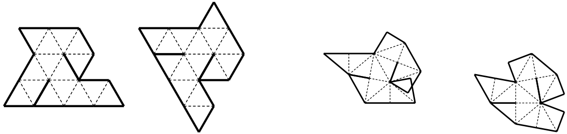
Figure 33 Pair 15 2 . Sunada triple G = \mathbf{PSL}(1, 2) , G_i = \langle a_i, b_i, c_i \rangle , i = 1, 2 , with a_1 = (0\ 14)(1\ 12)(2\ 6)(4\ 5)(7\ 11)(9\ 10) , b_1 = (1\ 13)(2\ 7)(4\ 6)(8\ 9) , c_1 = (0\ 12)(1\ 6)(3\ 5)(7\ 8) , a_2 = (0\ 11)(1\ 5)(3\ 4)(6\ 10)(8\ 9)(13\ 14) , b_2 = (0\ 10)(1\ 2)(6\ 9)(12\ 14) , c_2 = (0\ 13)(1\ 11)(2\ 3)(7\ 10) .
