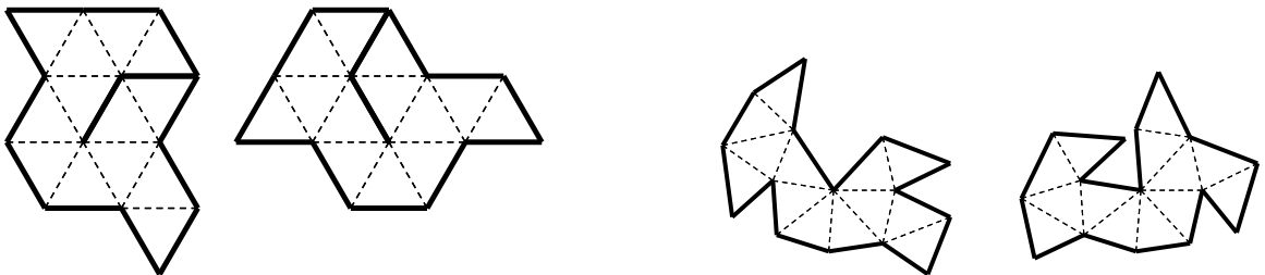
Figure 31 Pair 13 9 . Sunada triple G = \mathbf{PSL}(3,3) , G_i = \langle a_i, b_i, c_i \rangle , i = 1, 2 , with a_1 = (0\ 10)(1\ 5)(2\ 7)(3\ 12) , b_1 = (1\ 10)(3\ 6)(5\ 7)(9\ 11) , c_1 = (0\ 5)(1\ 2)(6\ 12)(9\ 11) , a_2 = (0\ 4)(1\ 6)(2\ 11)(9\ 12) , b_2 = (0\ 3)(2\ 4)(6\ 8)(7\ 11) , c_2 = (0\ 11)(1\ 8)(2\ 7)(3\ 4) .
