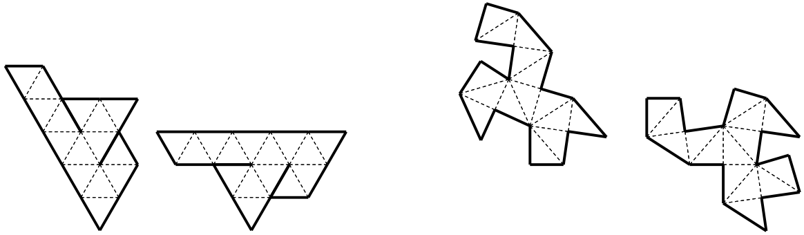
Figure 32 Pair 15 1 . Sunada triple G = \mathbf{PSL}(1, 2) , G_i = \langle a_i, b_i, c_i \rangle , i = 1, 2 , with a_1 = (0\ 14)(1\ 12)(2\ 6)(4\ 5)(7\ 11)(9\ 10) , b_1 = (1\ 13)(2\ 7)(4\ 6)(8\ 9) , c_1 = (1\ 14)(2\ 12)(3\ 4)(8\ 11) , a_2 = (0\ 11)(1\ 5)(3\ 4)(6\ 10)(8\ 9)(13\ 14) , b_2 = (0\ 10)(1\ 2)(6\ 9)(12\ 14) , c_2 = (0\ 5)(2\ 4)(6\ 7)(11\ 14) .
