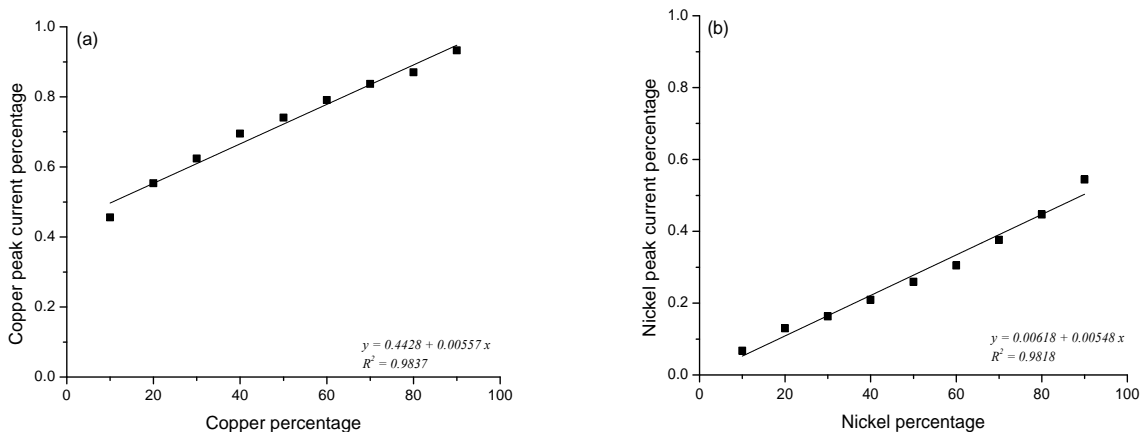
Figure 3. Dependence of copper and nickel oxidation peak current percentages on the composition of the copper-nickel alloy (total amount of the sample is 40 mg).
