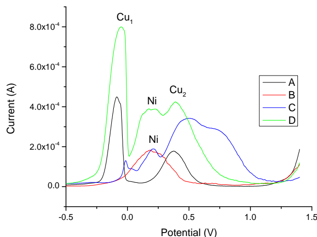
Figure 2. Differential pulse voltammograms of copper and nickel in potassium chloride solutions. (A and B) copper and nickel single electrodes, [KCl] = 3 M, scan rate 0.5 mV/s (optimum conditions). (C) copper and nickel mixture electrode, [KCl] = 0.68 M, scan rate 8.5 mV/s. (D) copper and nickel mixture electrode, in optimum conditions.
