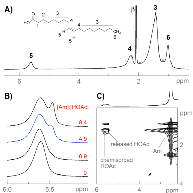
Figure 1. A) Bound HOAc (3-6) and toluene ( \beta ) are noted in the ^1H NMR spectrum of a HfO_2 NCs dispersion in toluene- d_8 , [HOAc] = 10.69 \text{ mol L}^{-1} . B) Upon addition of Am the alkene resonance splits in two parts, bound and free acid. C) 2D NOESY spectrum of HfO_2 NCs + 8.4 eq of Am.
