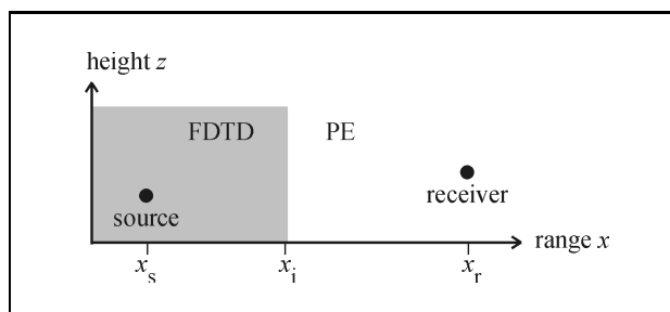
Figure 2. Geometry with xz coordinate system. The source region (gray area) extends to range x_i .
