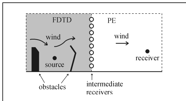
Figure 1. Schematic illustration of FDTD-PE model. FDTD is used in the source region (gray area), with complex obstacles and complex wind speed profiles. The FDTD computational domain is a little larger than the source region, so the intermediate receivers are located well within the FDTD computational domain. PE is used for propagation of the signals at the intermediate receivers to a distant receiver.
