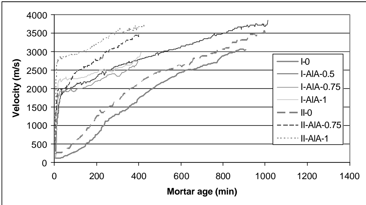
Fig. 2. Ultrasound velocity (hand picked onset time) vs. age for mortars containing the alkali-free accelerator AIS (top) or the alkali aluminate based accelerator AIA (bottom). Mortars were prepared using the cement types I 42.5 R (I) or CEM II/A-LL 42.5 R (II) and an accelerator dosage of 0, 0.5, 0.75 or 1 time the maximum allowable dosage of 50 ml per kg cement.
