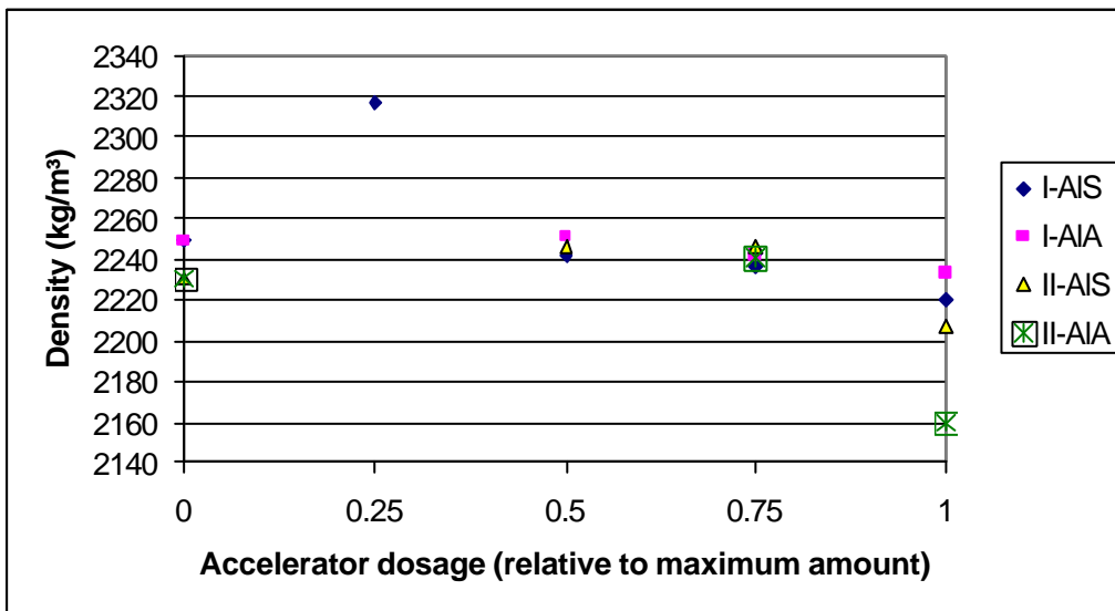
Fig. 6. Effect of accelerator type and dosage on the compressive strength, tensile strength in bending and density of the mortar prisms at 28 days (average standard deviation = 2.0 N/mm 2 for compressive strength, 0.18 N/mm 2 for tensile strength and 4.8 kg/m 3 for density)
