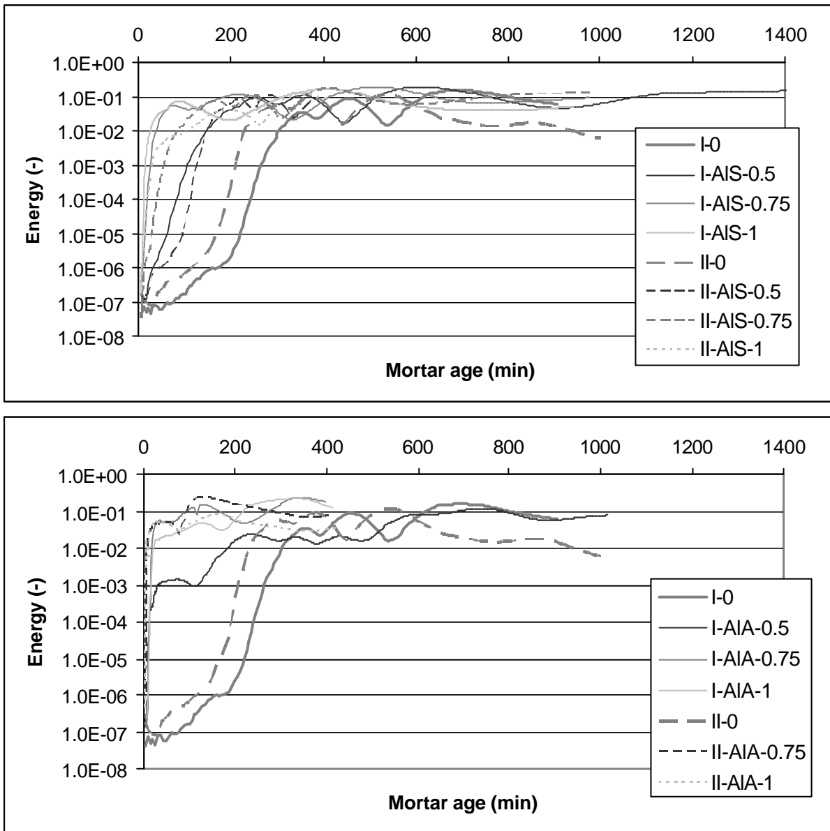
Fig. 3. Ultrasound energy vs. age for mortars containing the alkali-free accelerator AIS (top) or the alkali aluminat based accelerator AIA (bottom). Mortars were prepared using the cement types I 42.5 R (I) or CEM II/A-LL 42.5 R (II) and an accelerator dosage of 0, 0.5, 0.75 or 1 time the maximum allowable dosage of 50 ml per kg cement.
