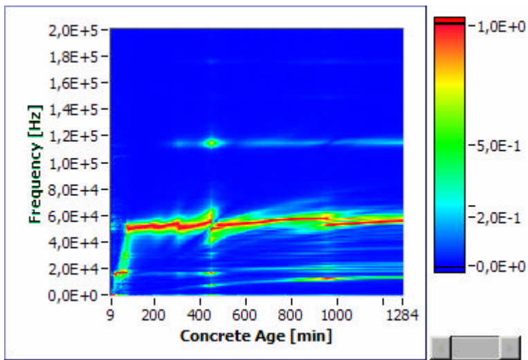
Fig. 5. Frequency content vs. age of the transmitted ultrasound signal for mortars I-0 (top) and I-AIS-0.5 (bottom)
