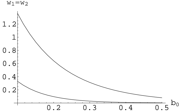
Figure 5: The solution \omega_1 = \omega_2 as a function of b_0 of eq.(B.92), top curve, and eq.(B.93), bottom curve, in units \Lambda_{\overline{\text{MS}}} = 1 . Clearly, these two curves do not coincide.
