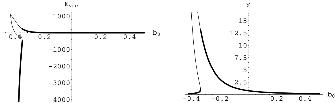
Figure 4: The vacuum energy E_{\text{vac}} and the expansion parameter y as a function of b_0 , in units \Lambda_{\overline{\text{MS}}} = 1 .
