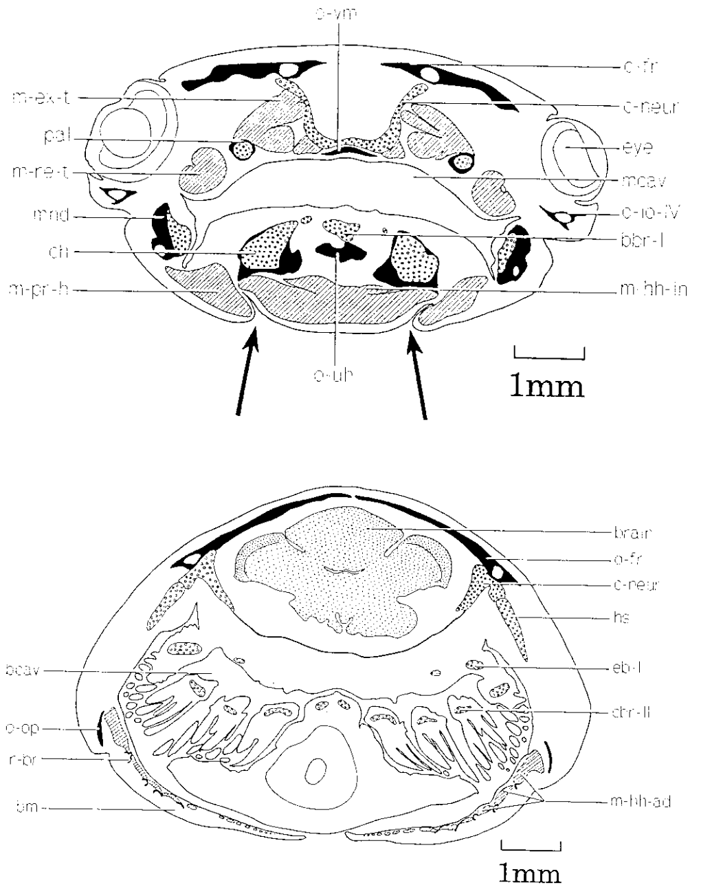
Fig. 6. — Cross section of juvenile C. gariepinus (SL = 46.75 mm): A. at the level of the eyes showing the small fold between the hyoid and the lower jaw (arrows); B. at the level of the anterior part of the opercular bone showing the firm, unfolded branchiostegal membrane (small circles indicate cartilage, black areas indicate bone, hatched areas indicate muscles).
