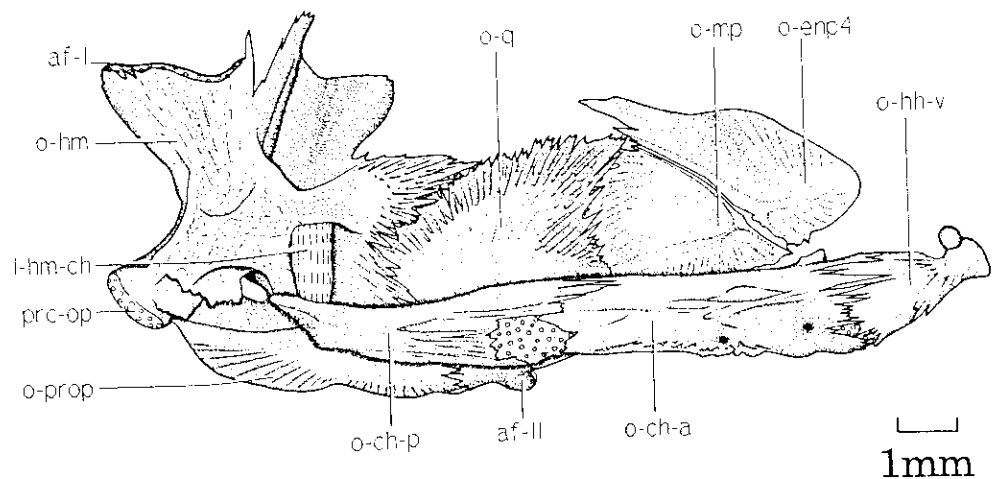
Fig. 4. — Medial view (left side) of suspensorium and hyoid of a juvenile C. gariepinus (SL = 136.20 mm) (small circles indicate cartilage).
