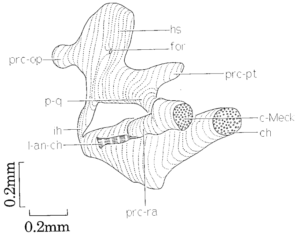
Fig. 1. — Graphical 3D-reconstruction : oblique, anterio-lateral view (right side) of cartilaginous suspensorium, lower jaw (partim) and ceratohyal (partim) of C. gariepinus (SL = 7.19 mm) (small circles indicate cartilage) (palatinum not drawn) (Abbreviations see page 152).
