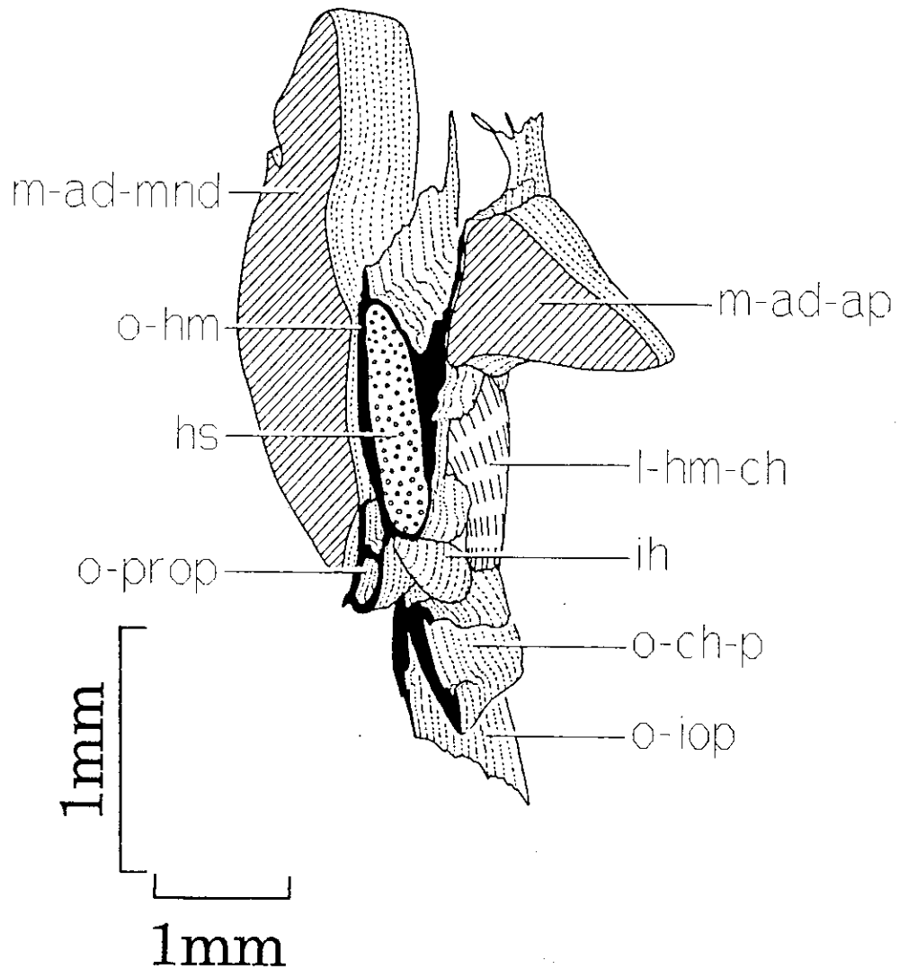
Fig. 2. — Graphical 3D-reconstruction : oblique, postero-medial view of the suspensorium (right side) at the level of the interhyal and the ligamentum hyomandibulo-ceratohyale of C. gariepinus (SL = 46.75 mm) (small circles indicate cartilage, black areas indicate bone, hatched areas indicate muscles).
