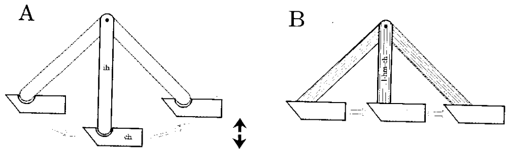
Fig. 5. — Scheme : A. rotation of the interhyal with a ventral excursion of the hyoid ; B. ligament replacing the interhyal with an anterior-posterior translation of the hyoid.
