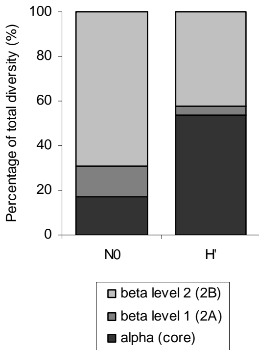
Figure 6: Stacked columns depicting the composition of the gamma diversity and the proportions of the alpha diversity and different beta diversity levels (between replicate cores, between habitats) in the Håkon Mosby Mud Volcano. Diversity was measured as genus richness based on presence-absence data, and the Shannon-Wiener index based on abundance data.
