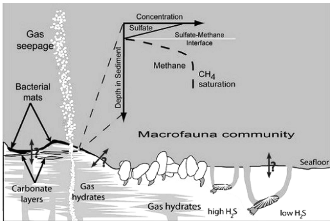
Figure 2: Scheme of biogeochemical relationships at seep locations illustrating the chemosynthetic megafauna and microbial mats, including a graph concerning sulphate and methane concentration in relation to sediment depth 3 .
