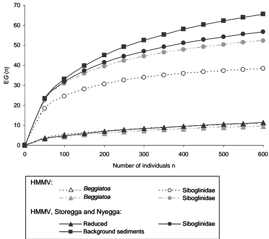
Figure 8: Rarefaction curves for the pooled data per habitat at three different spatial scales. White symbols represent the micro-scale (only at Håkon Mosby Mud Volcano, HMMV), grey symbols represent the macro-scale (only at HMMV), and black symbols represent the mega-scale (HMMV, Storegga Slide, Nyegga pockmarks).
