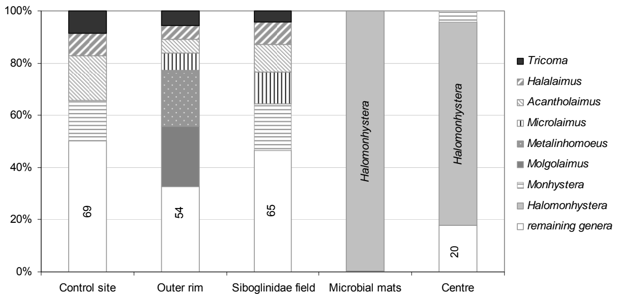
Figure 7: Proportional abundance of the most abundant nematode genera at the different sites inside and outside HMMV (numbers in white bars are number of remaining genera).
