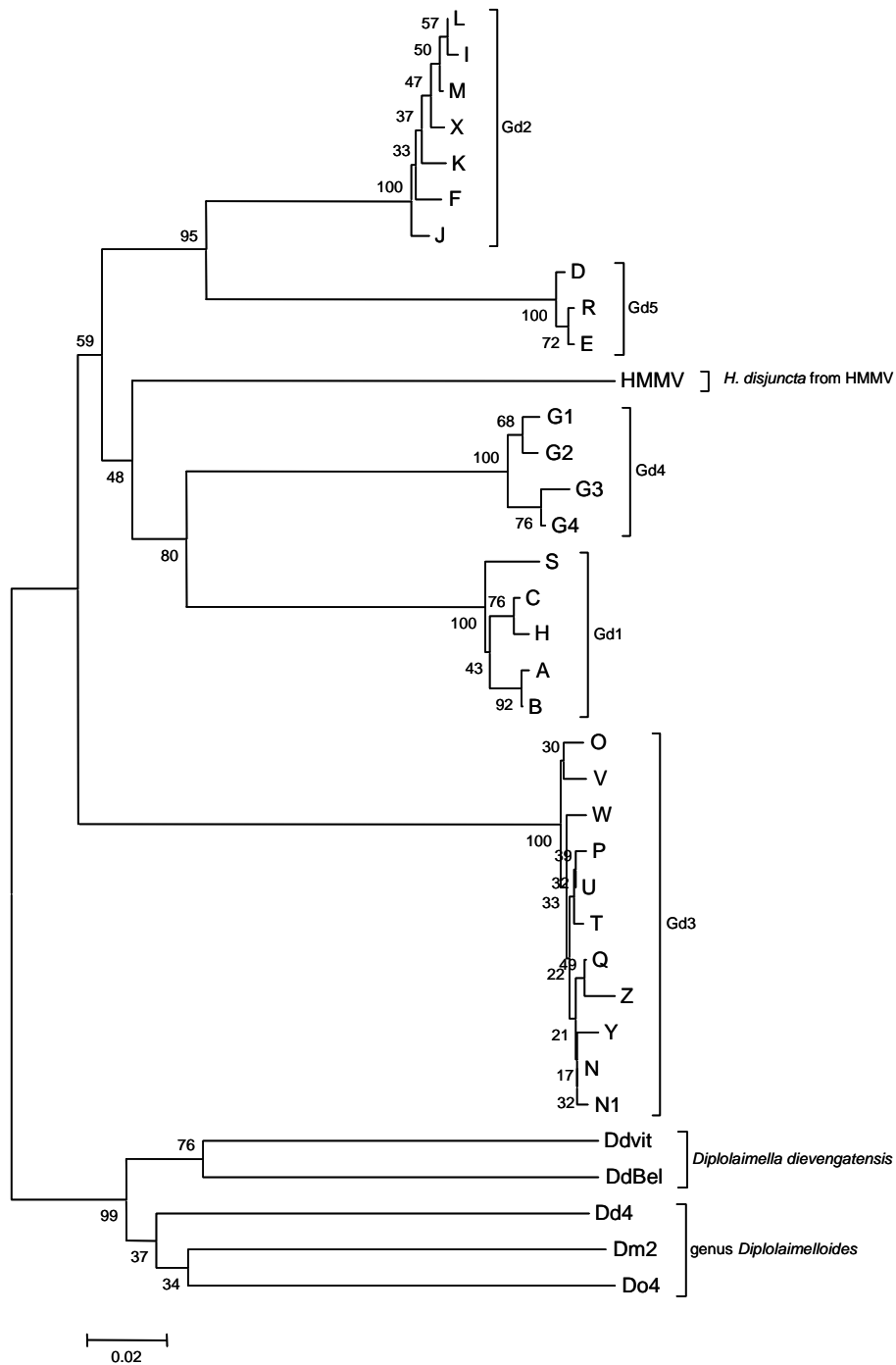
Figure 6: Phylogenetic position of HMMV among cryptic species of the Halomonhystera disjuncta species complex from Derycke et al. (2007). The closely related monhysterids Diplolaimelloides meylli , D. oschei , D. deleyi and Diplolaimella dievengatensis were used as outgroup. NJ tree of COI haplotypes with branch lengths calculated on the basis of P-distances. Bootstrap values are based on 1000 replicates.
