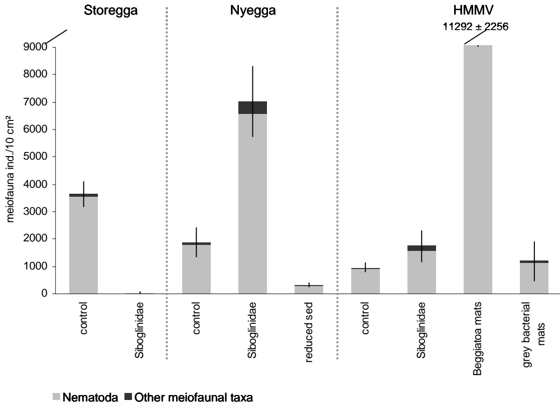
Figure 2: Mean total densities of meiofauna in the different habitats at Storegga Slide (740 m), Nyegga area (730 m) and Håkon Mosby Mud Volcano (1280 m) (mean \pm 1 SD).
