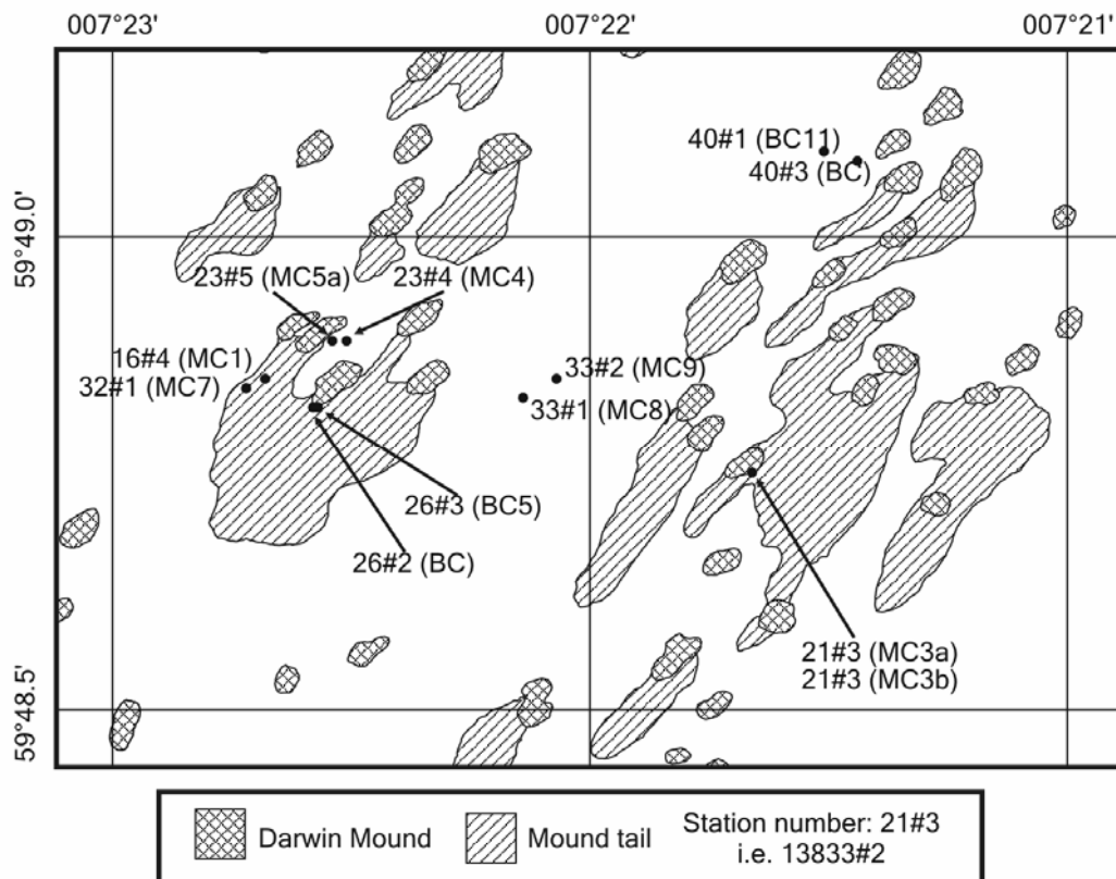
Figure 2: A detailed view of the Darwin Mounds sampling sites shown on a simplified interpretation of sidescan sonar imagery (adapted from Masson et al. 2003).
