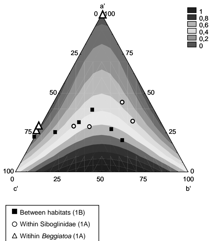
Figure 5: Ternary plot of the turnover of nematode genera at Norwegian seeps at the micro-scale. Turnover rates rang from 0 to 1, where 1 represents the complete turnover of genera.
