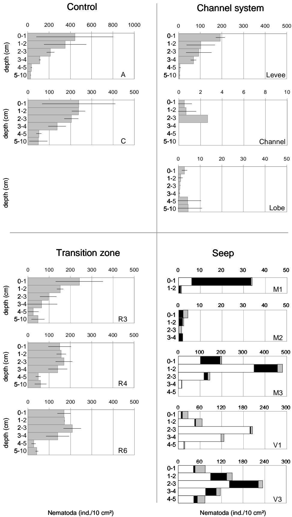
Figure 5: Depth profiles of nematode densities for the different sites (ind. 10 cm -2 ) (mean values ± 1 SD) (in seep profiles: white bars = Sabatieria mortensenii ; black bars = Desmodora sp.; grey bars = remaining genera).
