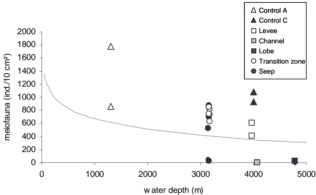
Figure 4: Average meiofaunal densities of the different sites in the Gulf of Guinea arranged according to water depth (m), compared with the best regression line [ y = 2821.76 - 286.86 * (\ln \text{depth}) ] from Soltwedel (1997) for the continental margins off the western African coast between Guinea (10°N) and Angola (18°S).
