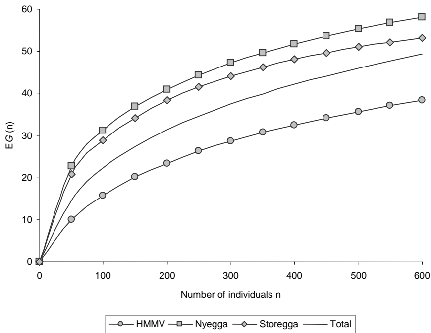
Figure 9: Rarefaction curves for the pooled data per sampling area at the Norwegian continental margin, and for the complete region.
