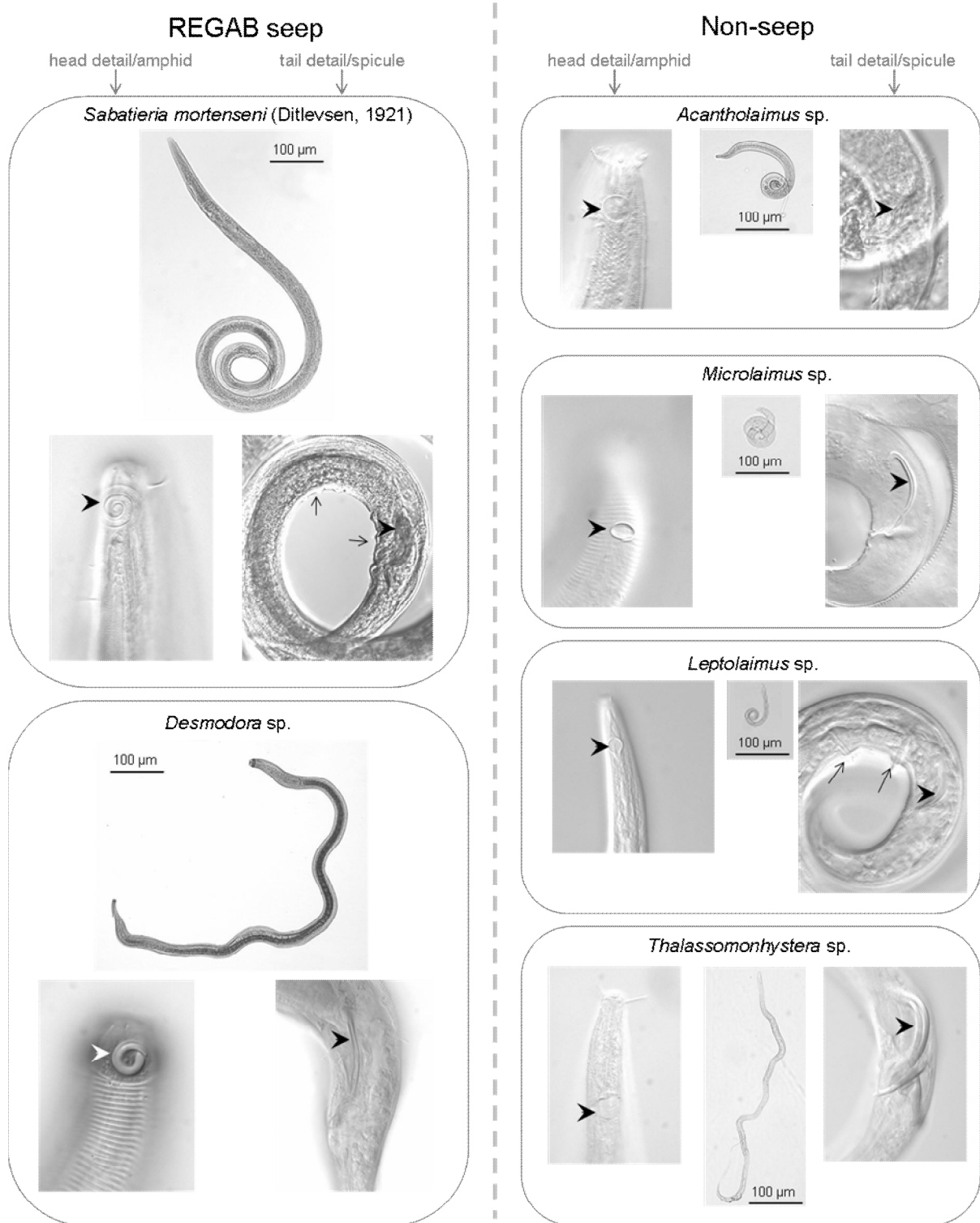
Figure 6: Overview of the dominant nematodes (males) in the seep site and in the non-seep sites in the Gulf of Guinea. Photographs on the left show the two dominant nematode species from REGAB, photographs on the right show representative species for the four most abundant nematode genera in the non-seep sites. Photographs of the nematode habitus are all placed on the same scale. Closed arrows point to the amphid at the anterior part or the spicule at the posterior part of the nematode, open arrows point to the preloocal supplements.
