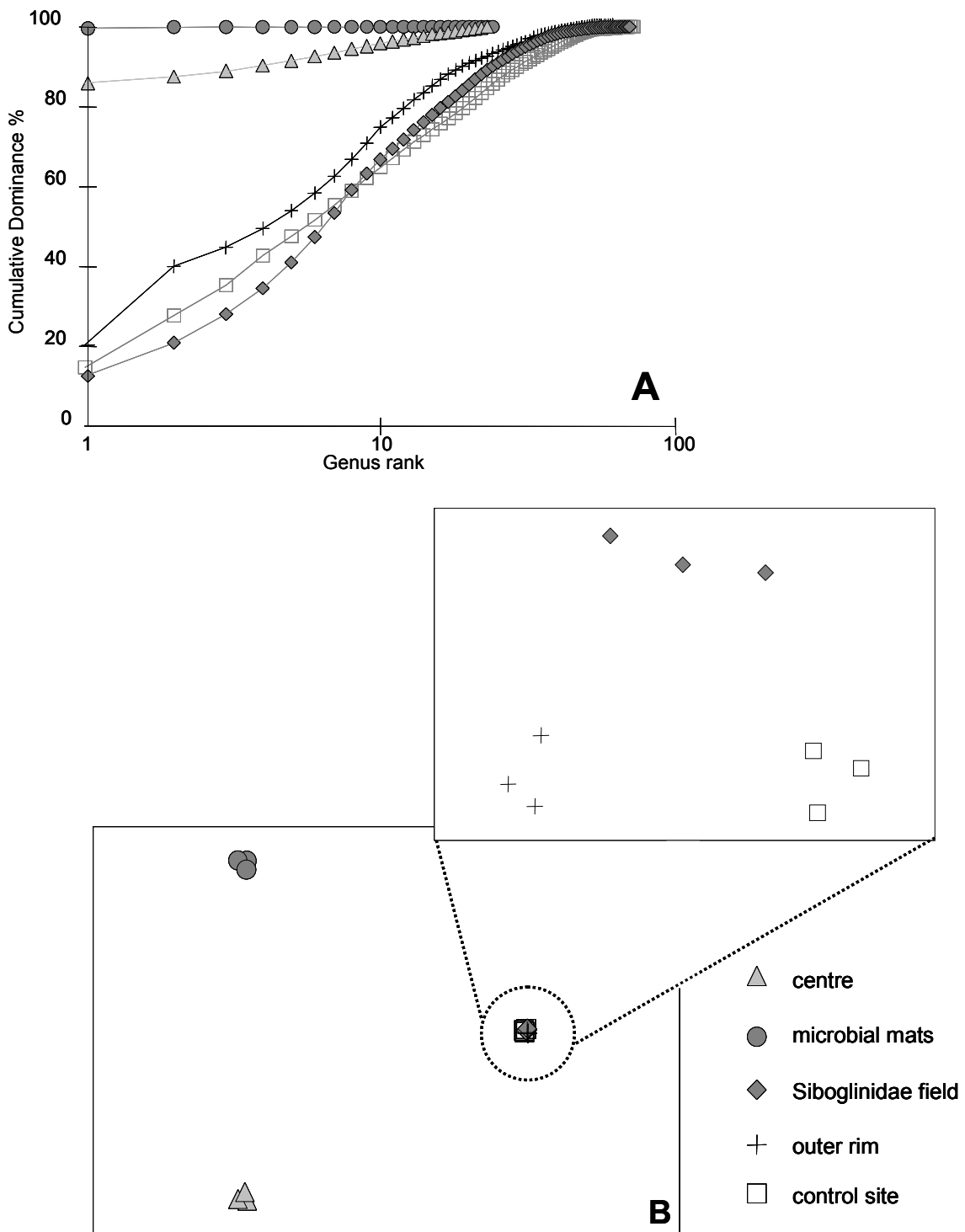
Figure 8: (a) K -dominance curve of all nematode genera found at the different sites and (b) nonmetric-multidimensional scaling plots based on nematode genus densities. Plot in background is based on all sites, plot on foreground displays only the control sites, outer rim sites and Siboglinidae sites.
