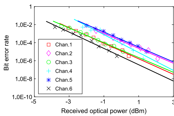
Fig. 9. Bit error rate for the transmitter at 12.5 Gb/s using the setup shown in Fig. 5(a) by replacing the DCA with a real-time oscilloscope.
