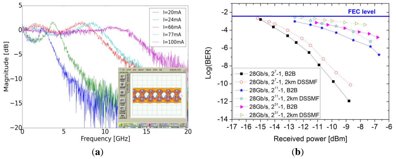
Figure 7. (a) Small signal response at different bias currents and large signal eye diagram at 28 Gbps with 2.1 dB extinction ratio using 2^{11} -1 pattern length (inset). (b) bit error ratio (BER) measurements for back-to-back and 2 km DSSMF configuration. Reproduced from [26].
