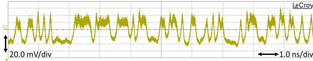
Figure 15. Large signal modulation response of a full optical link based on a microdisk laser, an SOI waveguide and a heterogeneously integrated photodetector for a 10 Gbps 2^7-1 PRBS pattern. Reproduced from [52]. © 2013 IEEE
