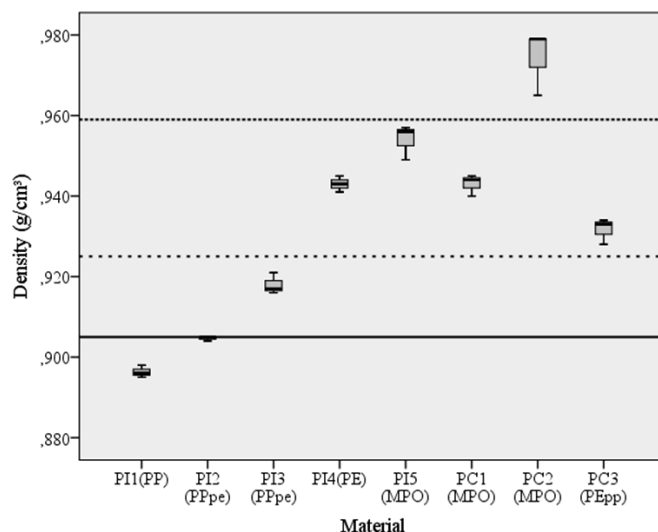
Figure 2. Density values of polyolefin waste materials.
